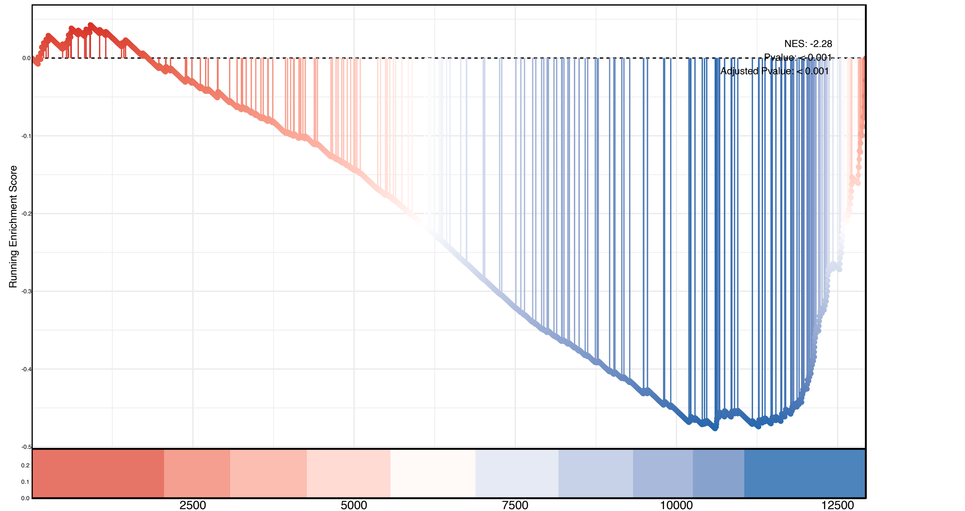
Microtubule Binding
