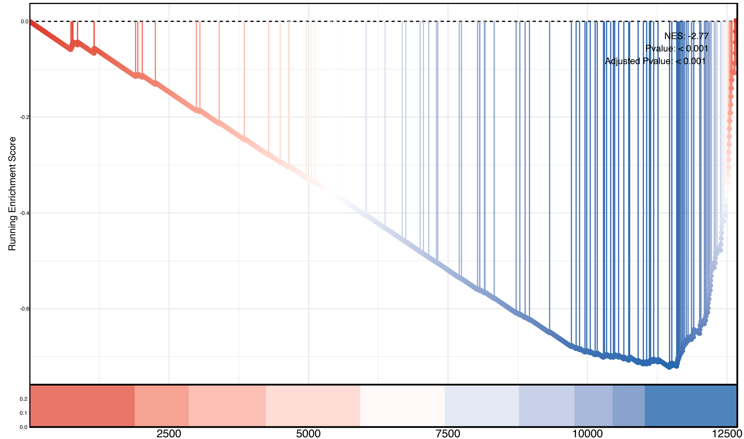
Late Up.v1 Up
