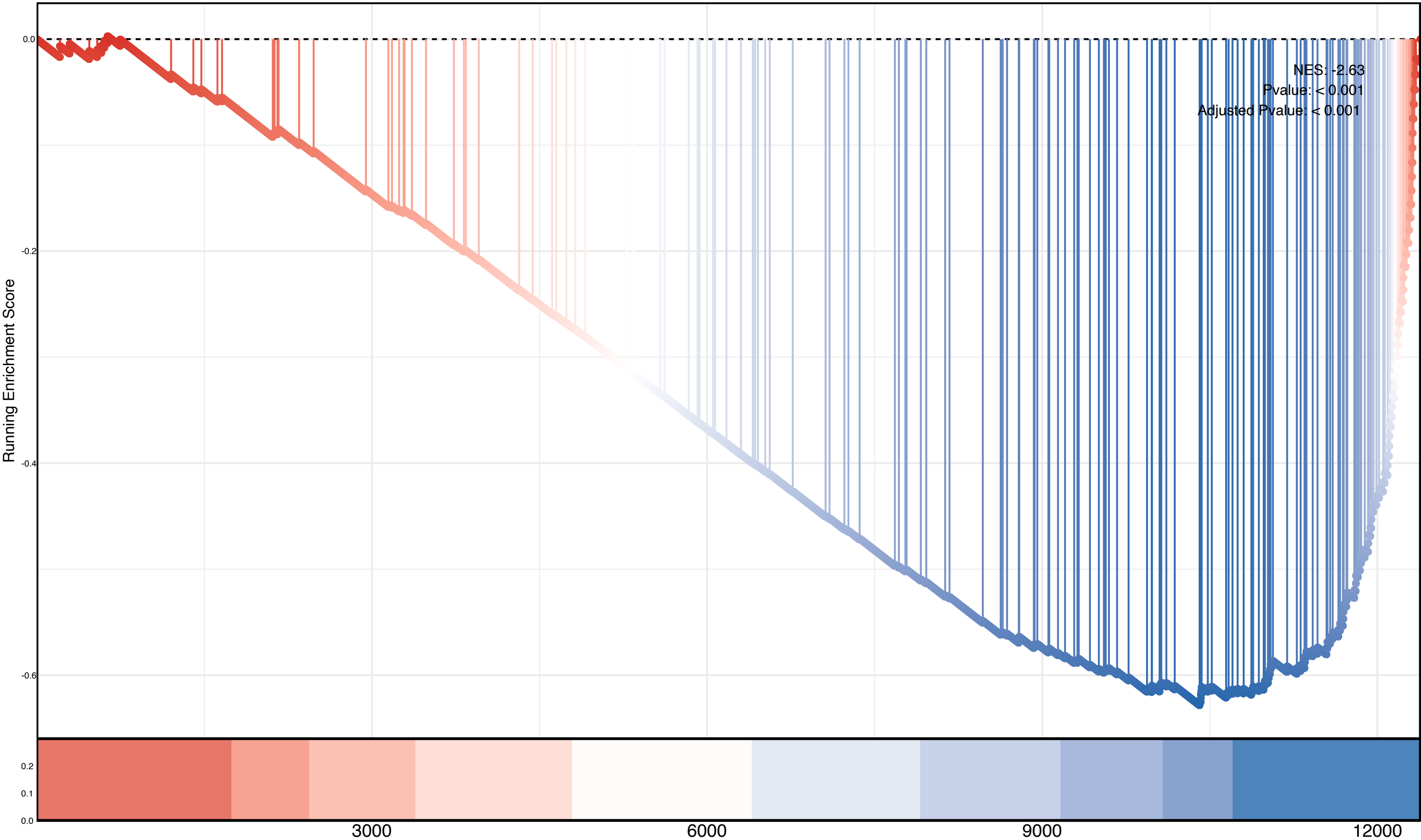
Mitotic Sister Chromatid Segregation
