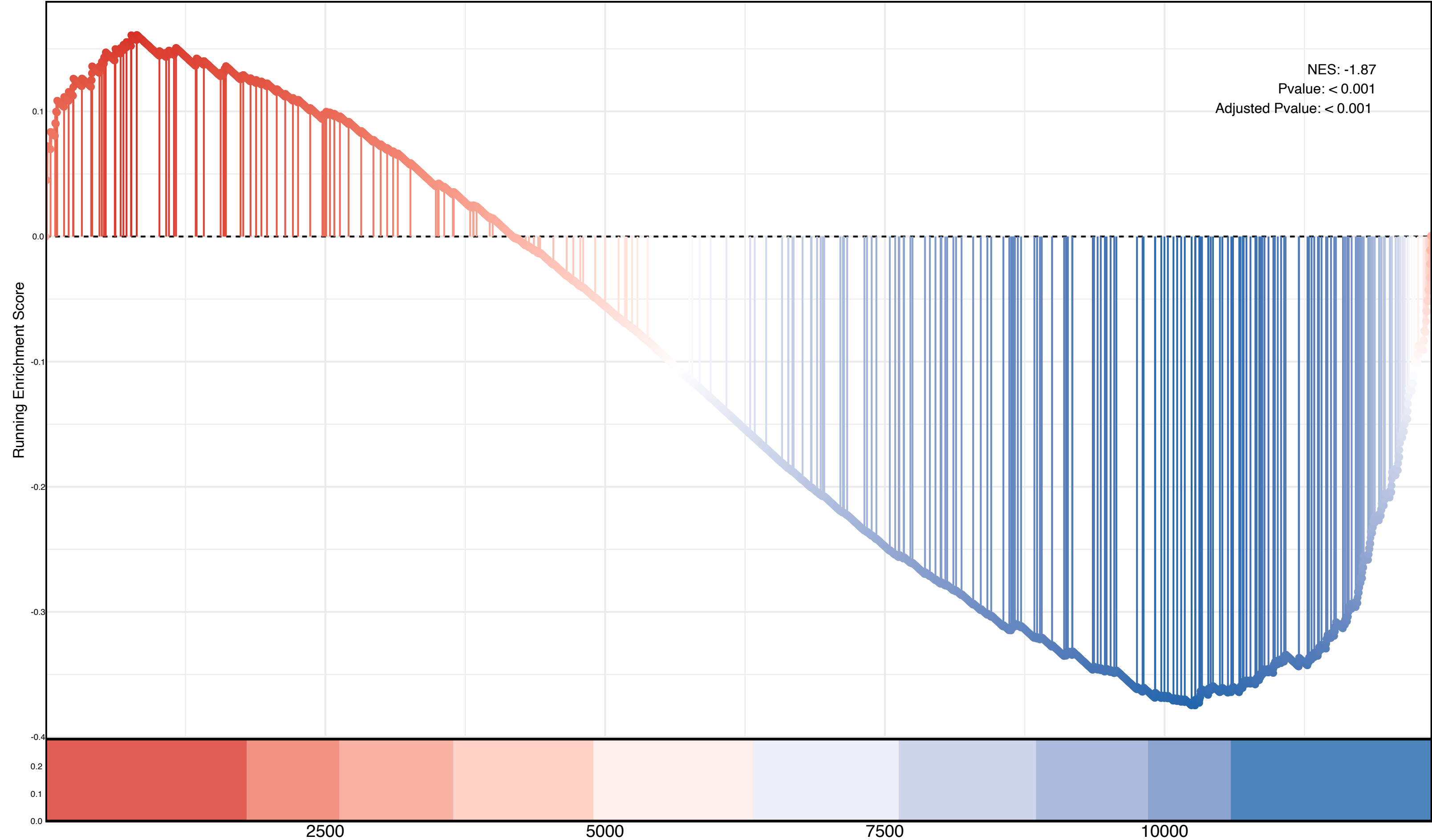
Mirtargeted Genes In Muscle Cell
