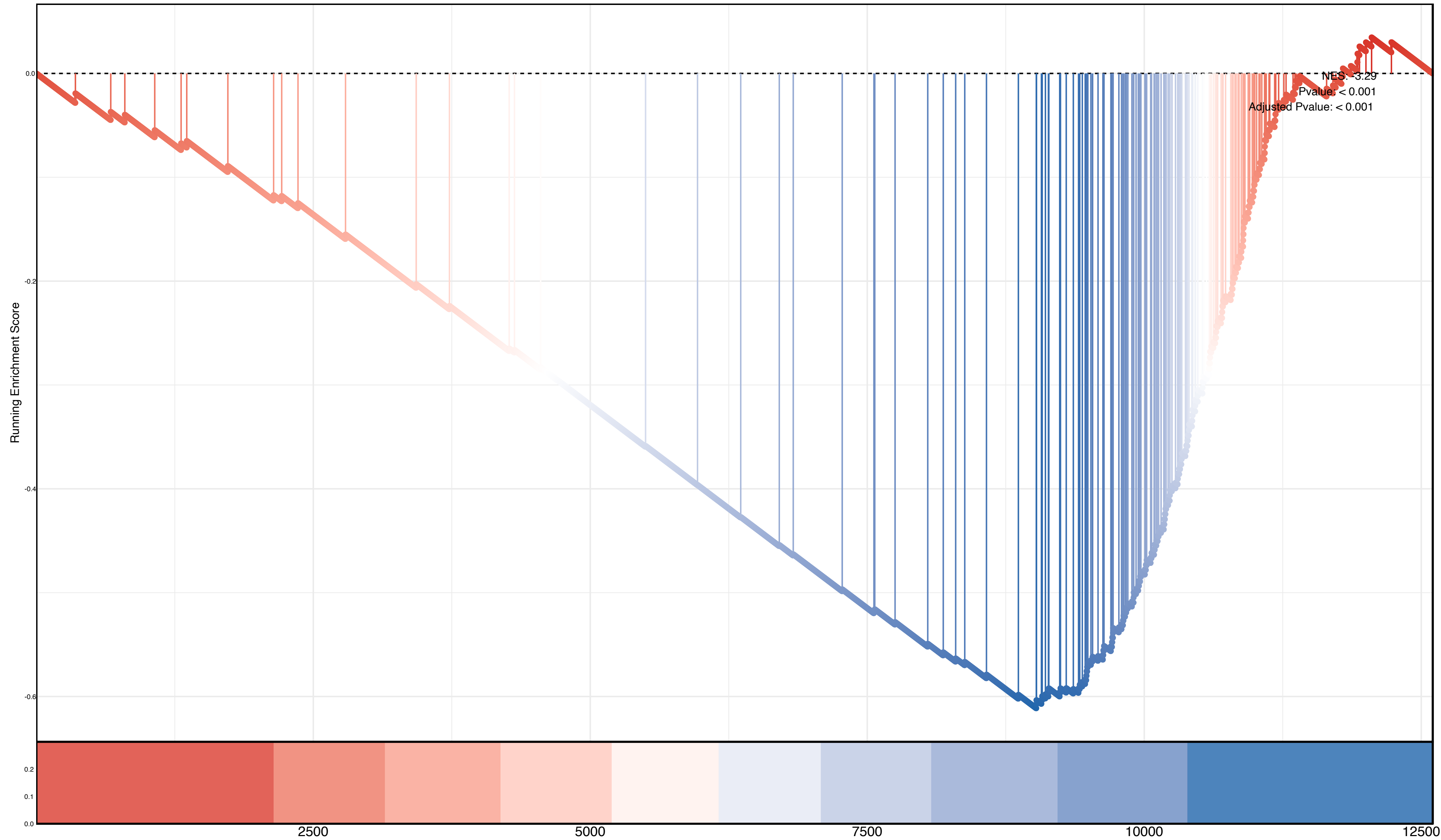
Day6 Vs Day10 Eff Cd8 Tcell Up
