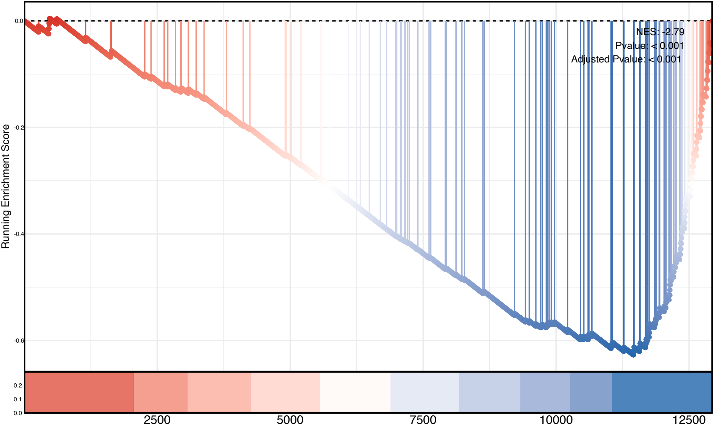
Mitotic Spindle Organization
