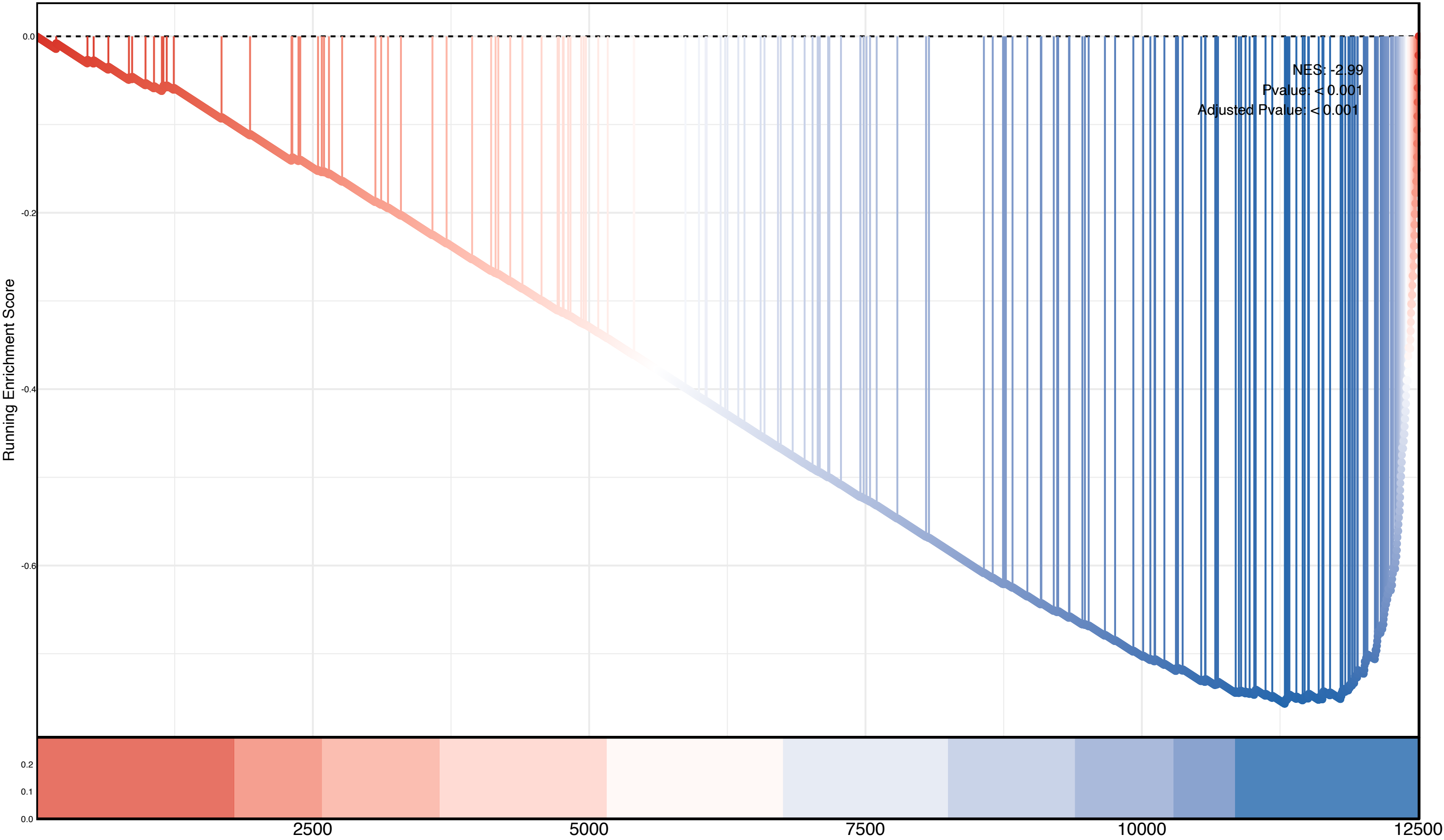
Sister Chromatid Segregation
