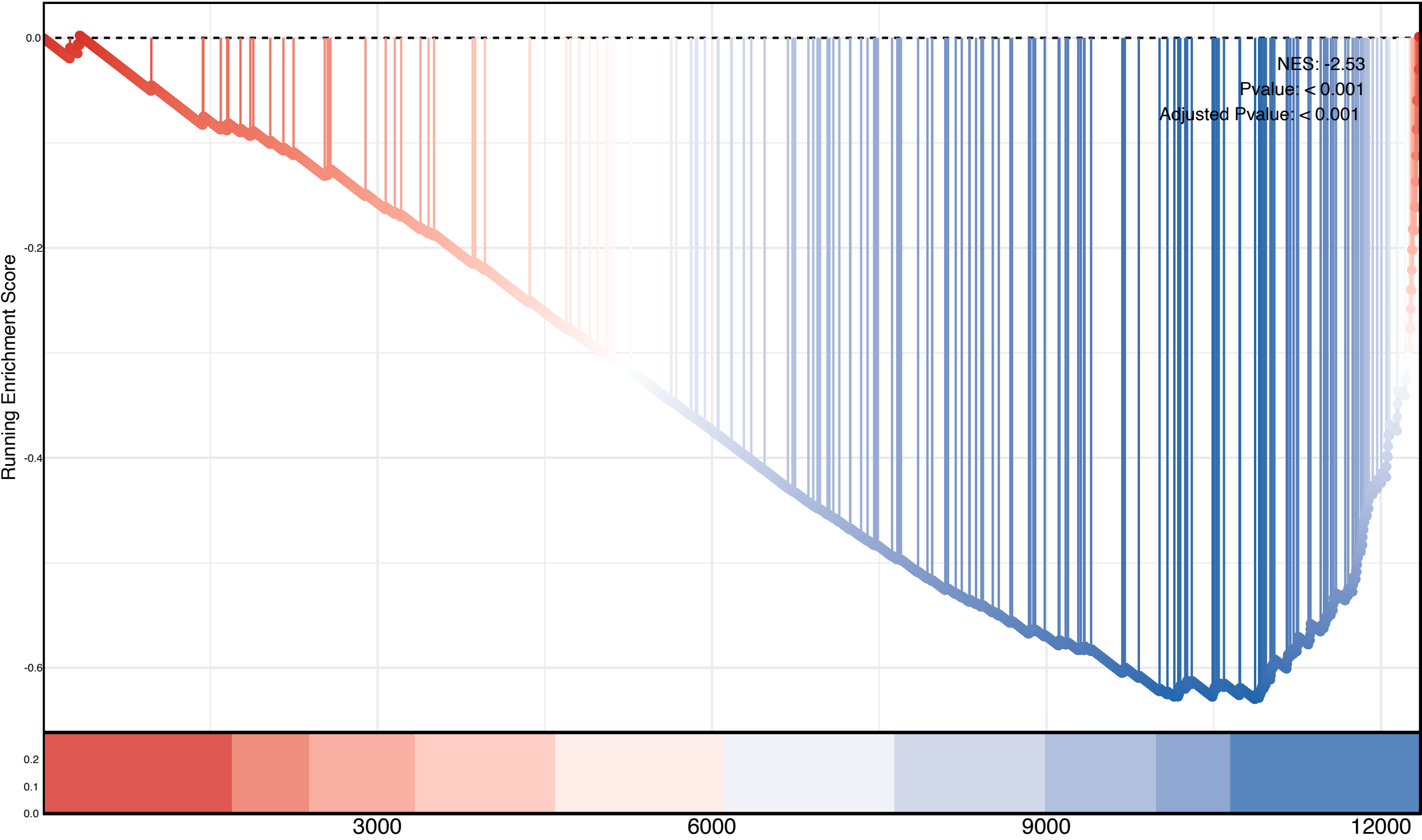
Nuclear Chromosome
