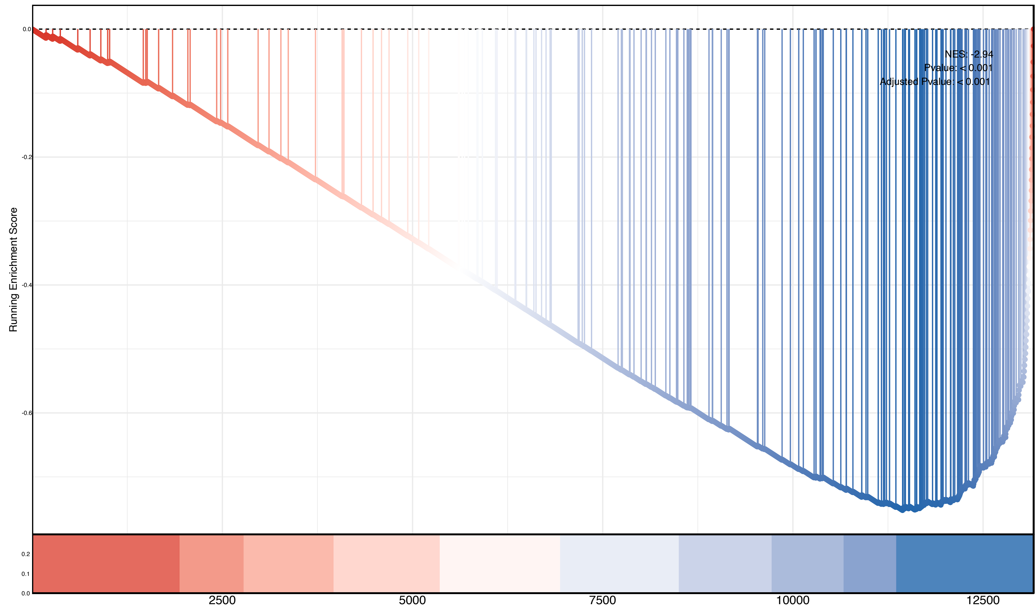
Regulation Of Chromosome Organization
