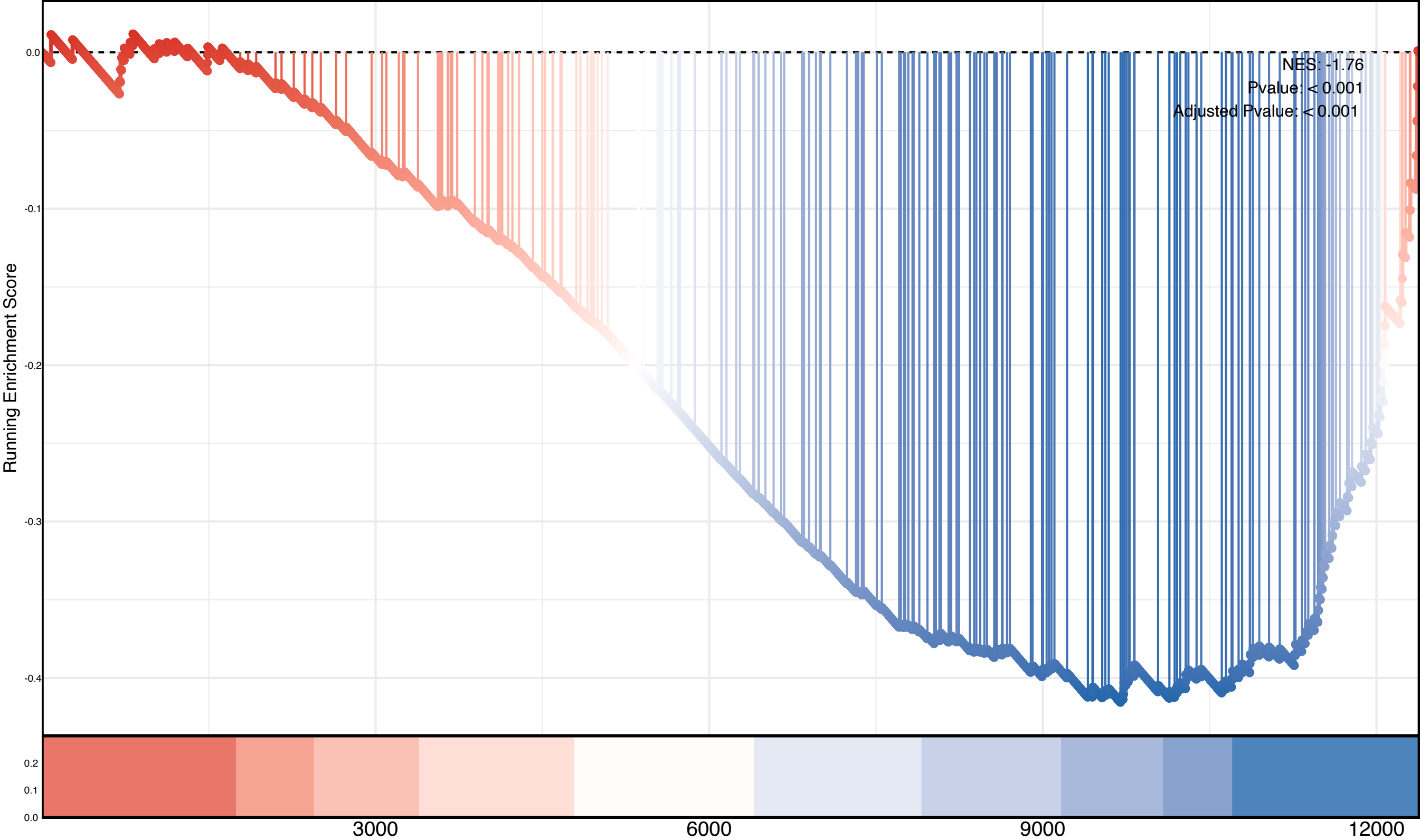
Protein Heterodimerization Activity
