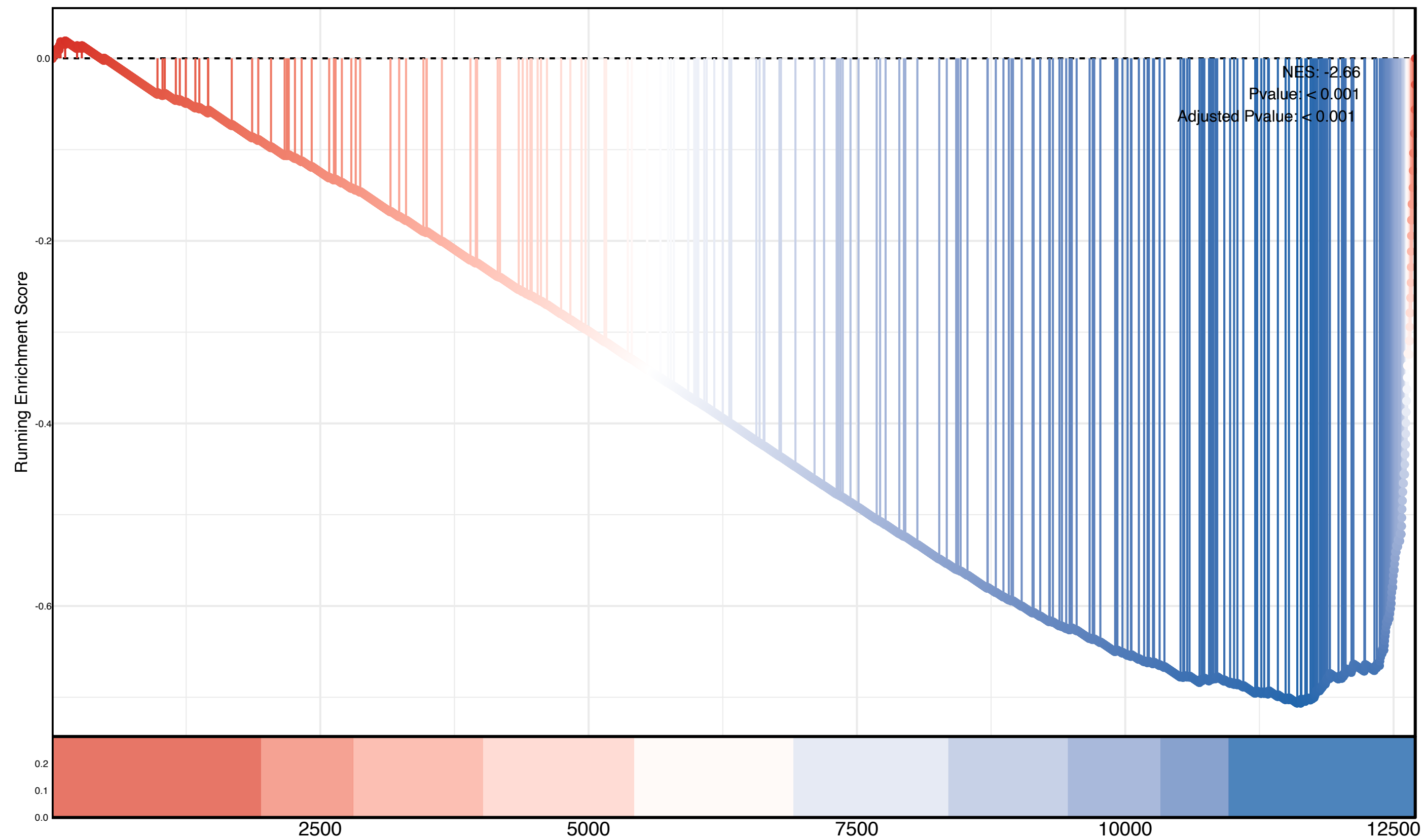
Cell Cycle Checkpoints
