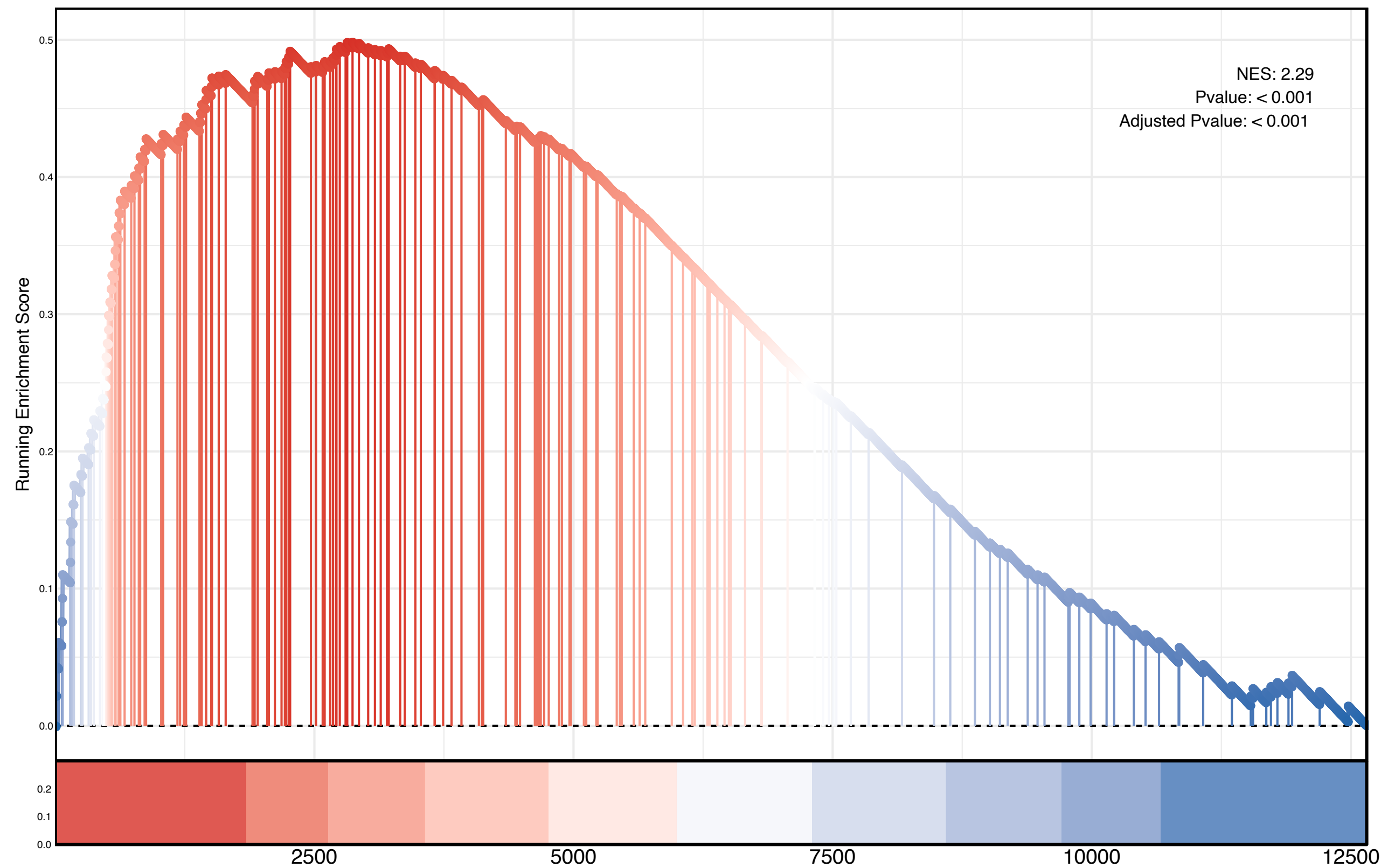
Ctrl Vs 12h F Tularensis Lvs Neutrophil Dn
