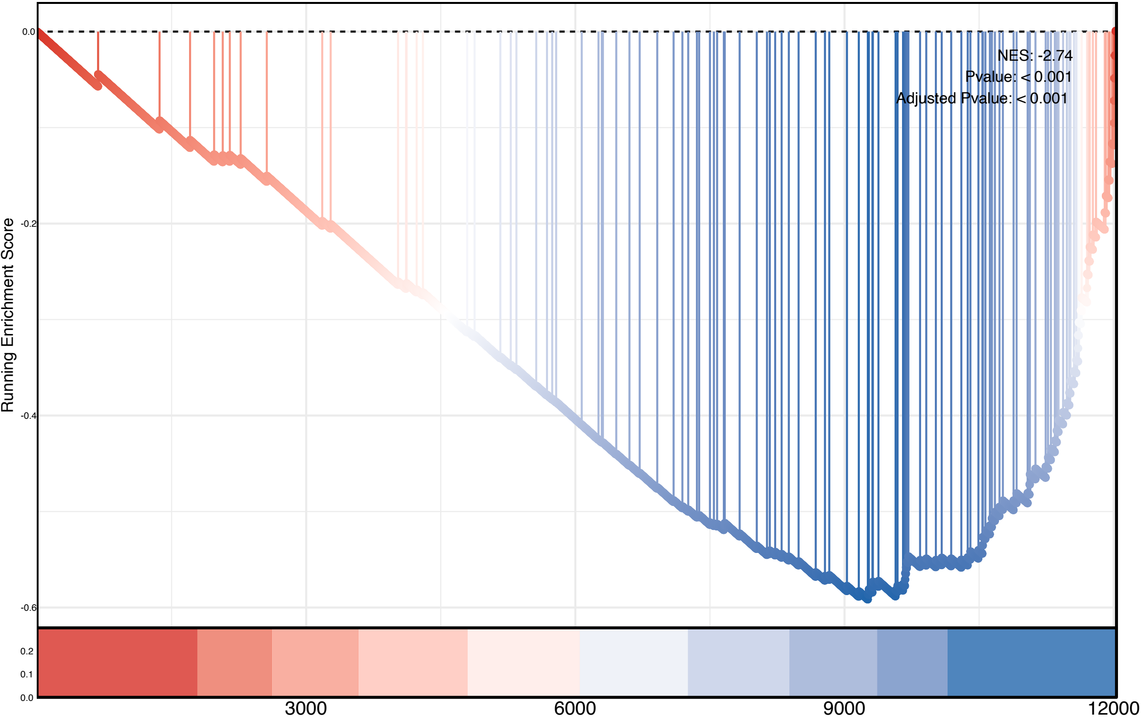
Regulation Of Mrna Processing
