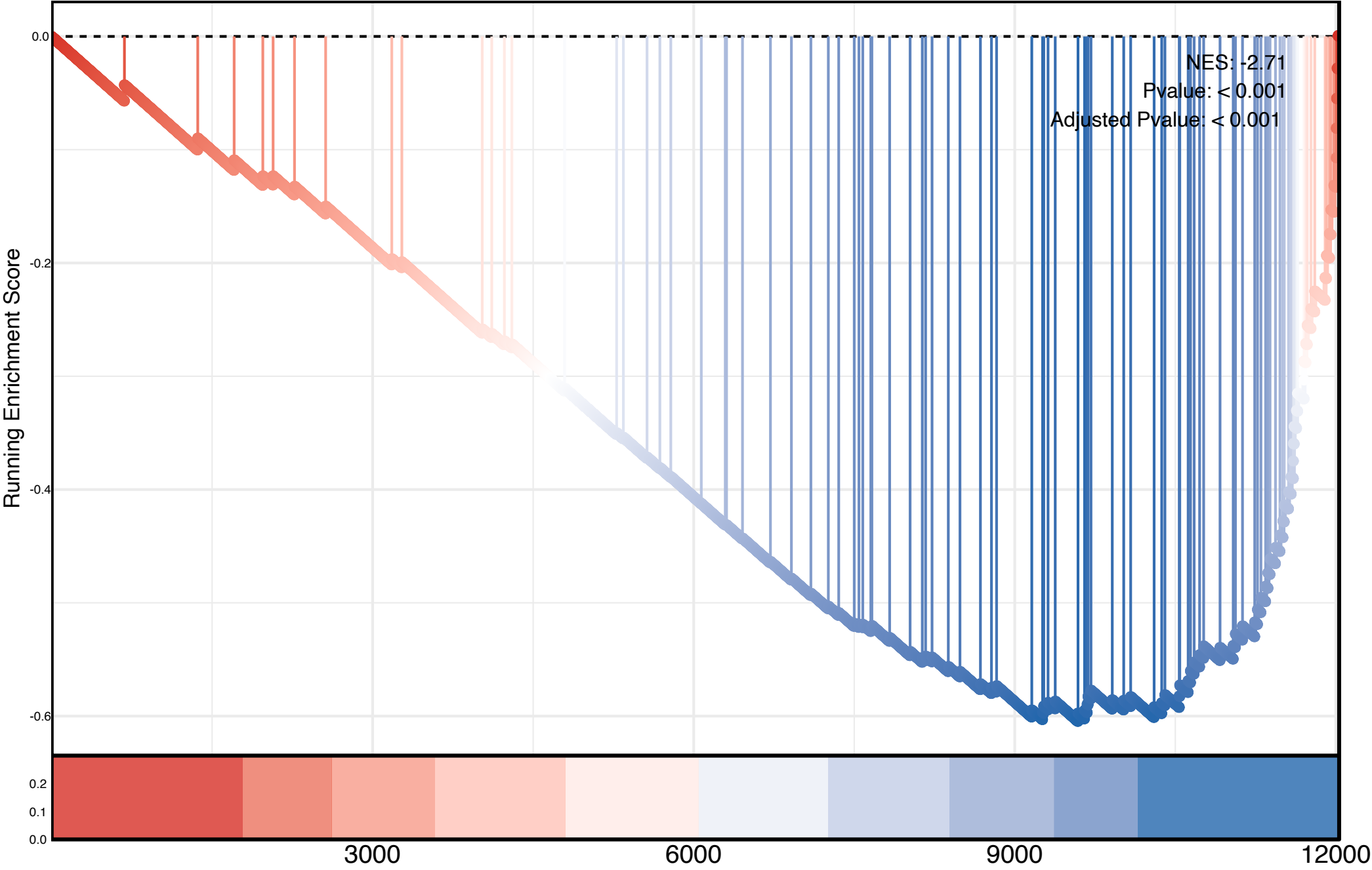
Regulation Of Mrna Splicing Via Spliceosome
