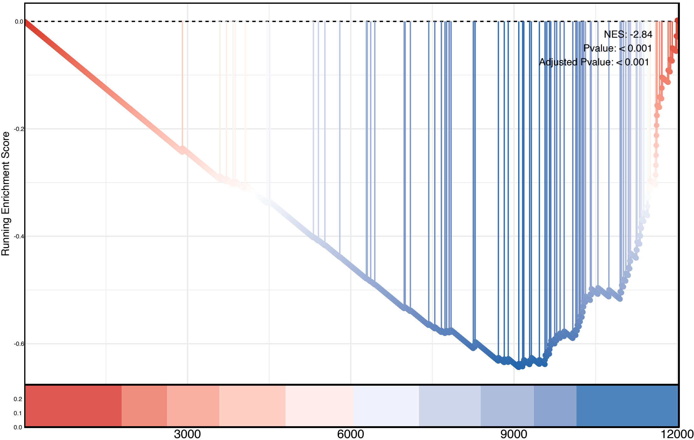
Sm Like Protein Family Complex
