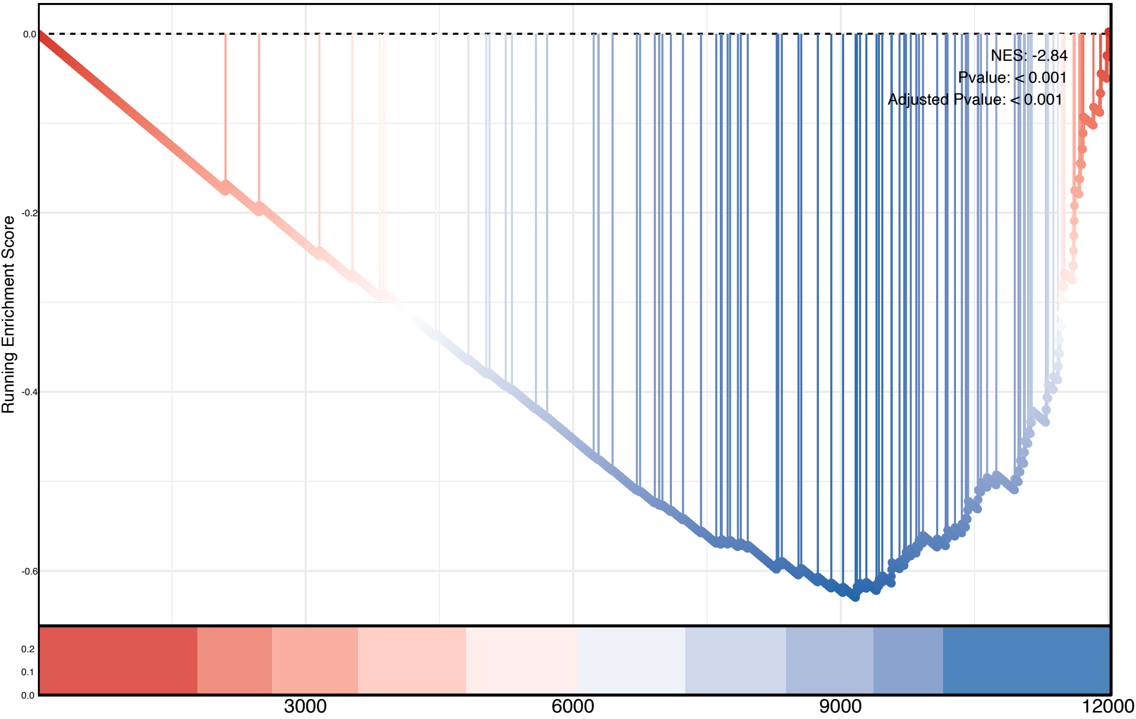
U2 Type Spliceosomal Complex
