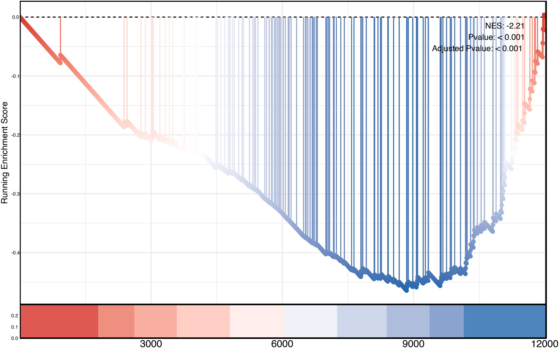
Structural Constituent Of Ribosome
