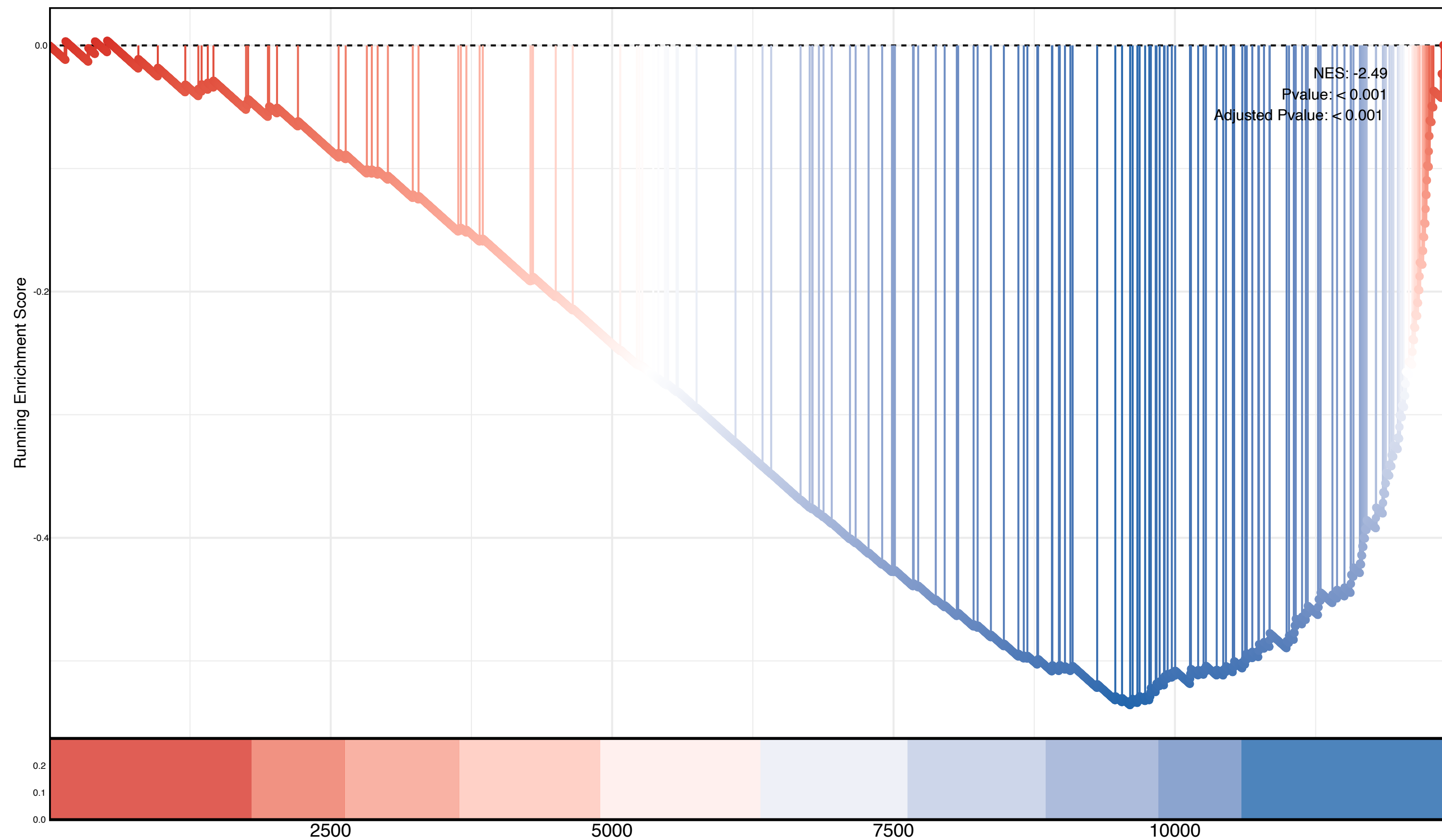
Day6 Effector Vs Day30 Exhausted Cd8 Tcell Lcmv Clone13 Dn
