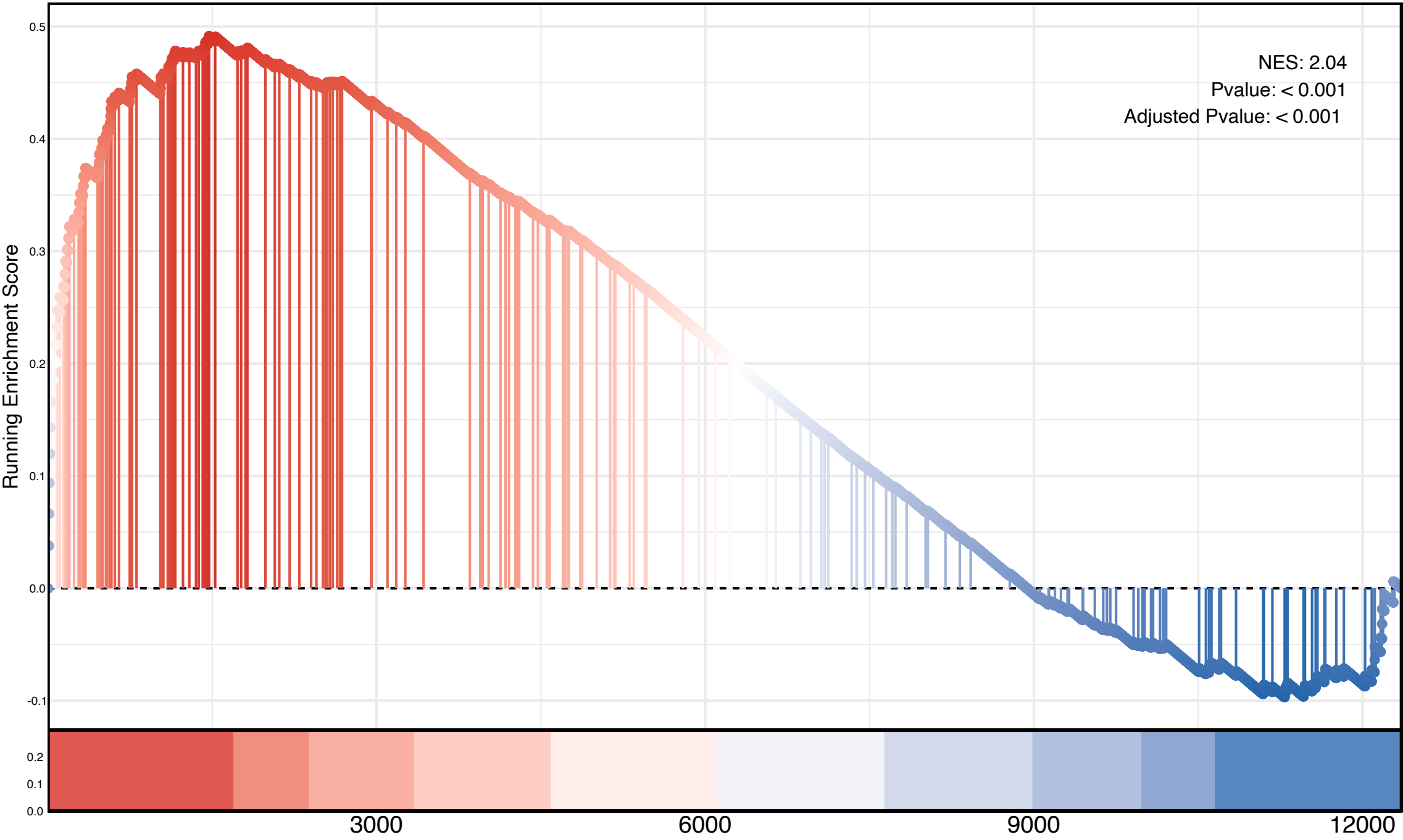
Nuclear Receptors Metapathway
