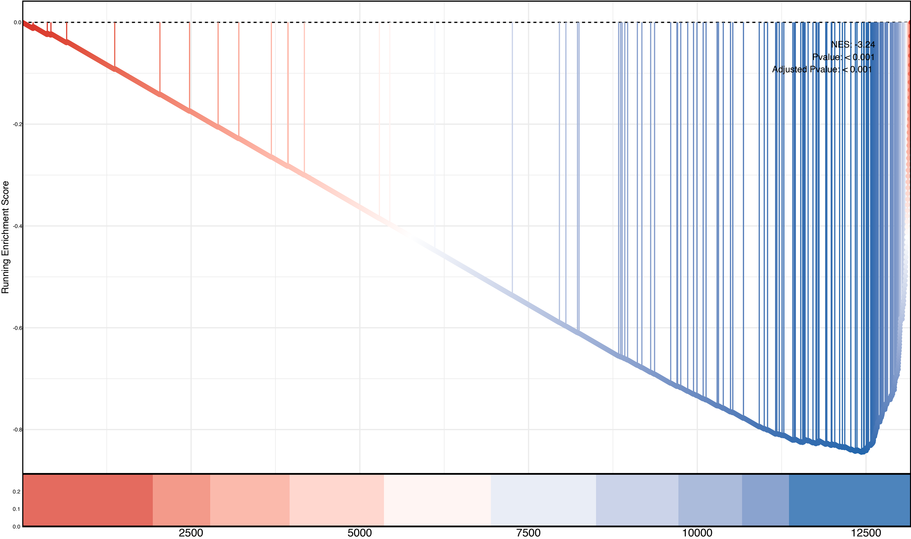
G2m Checkpoint
