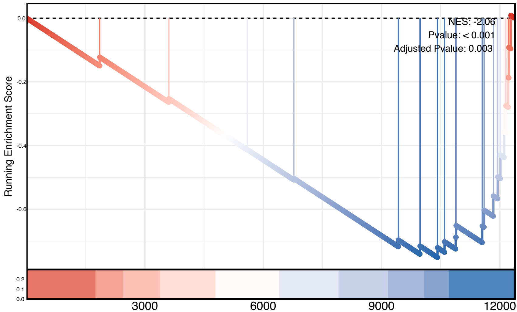
Medicus Reference Condensin Loading
