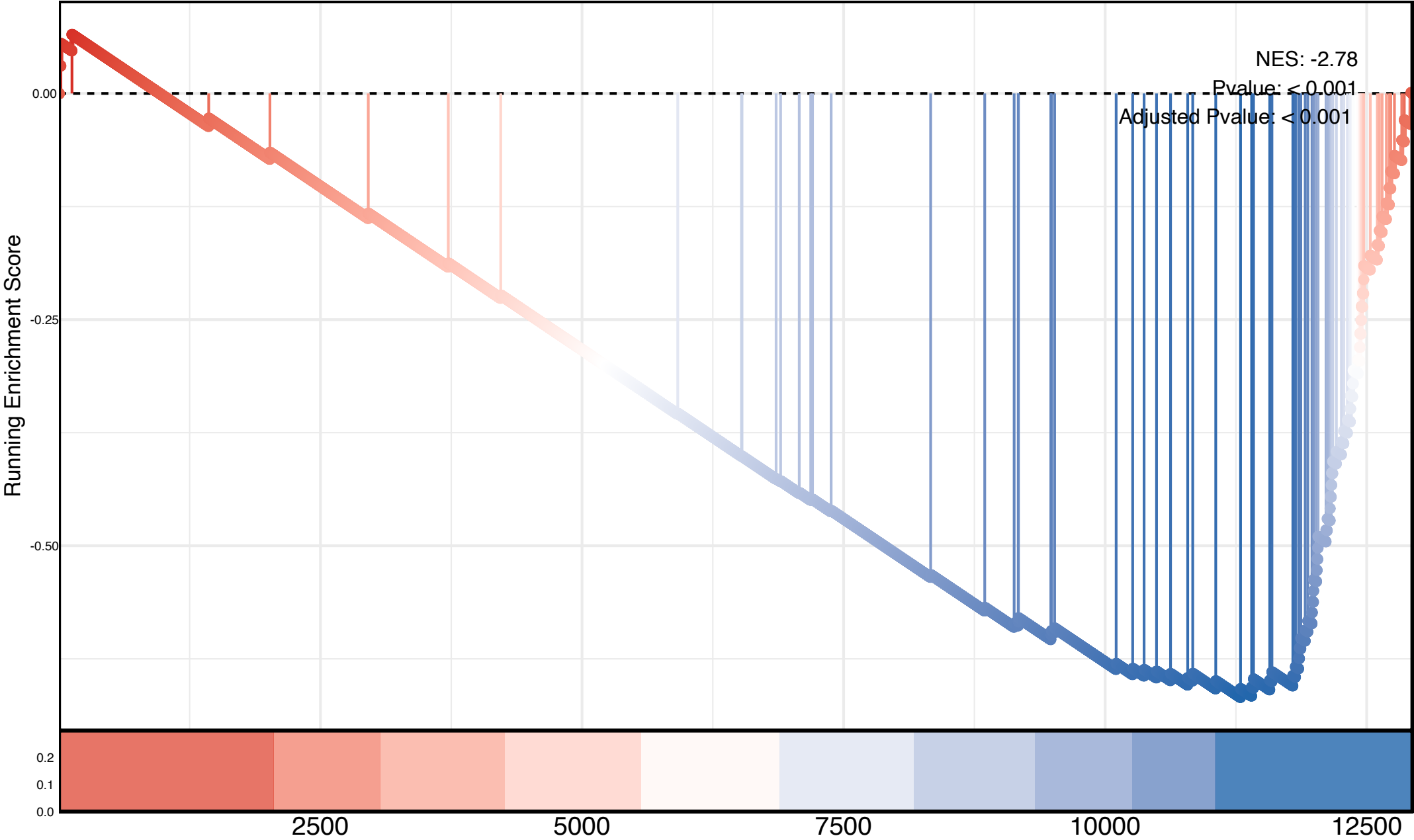
Chromosome Separation
