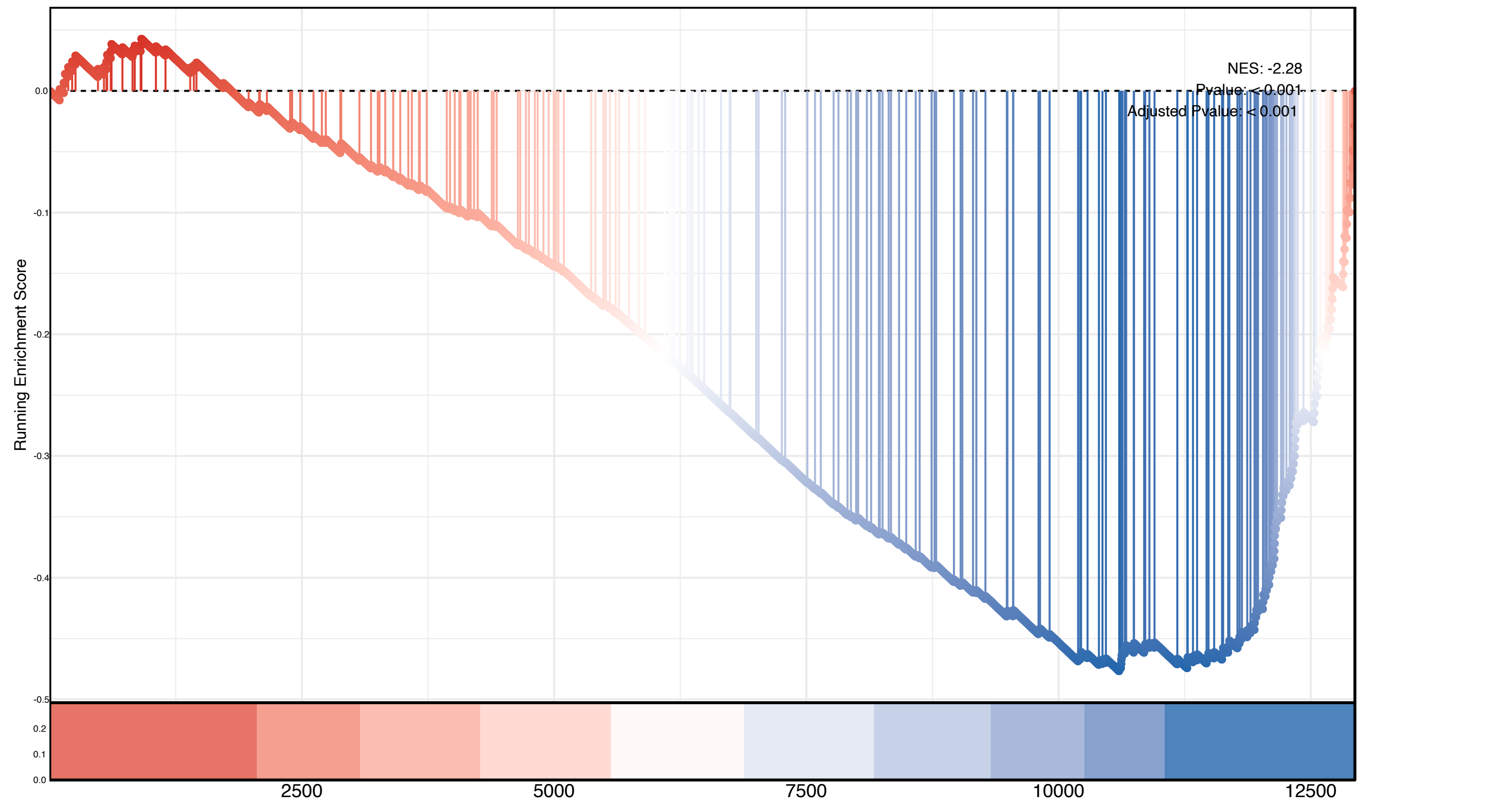
Microtubule Binding
