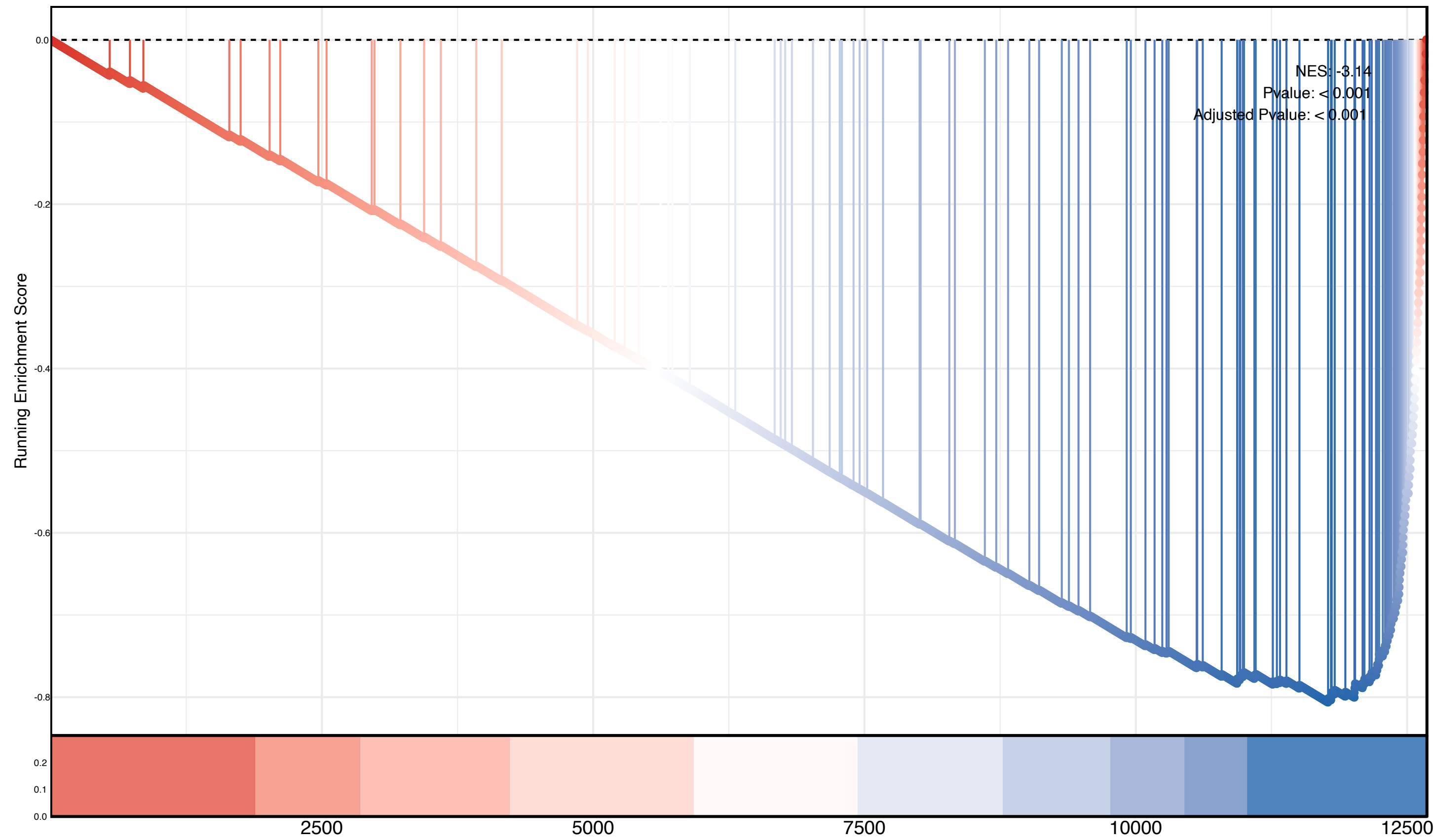
Induced Vs Natural Treg Dn
