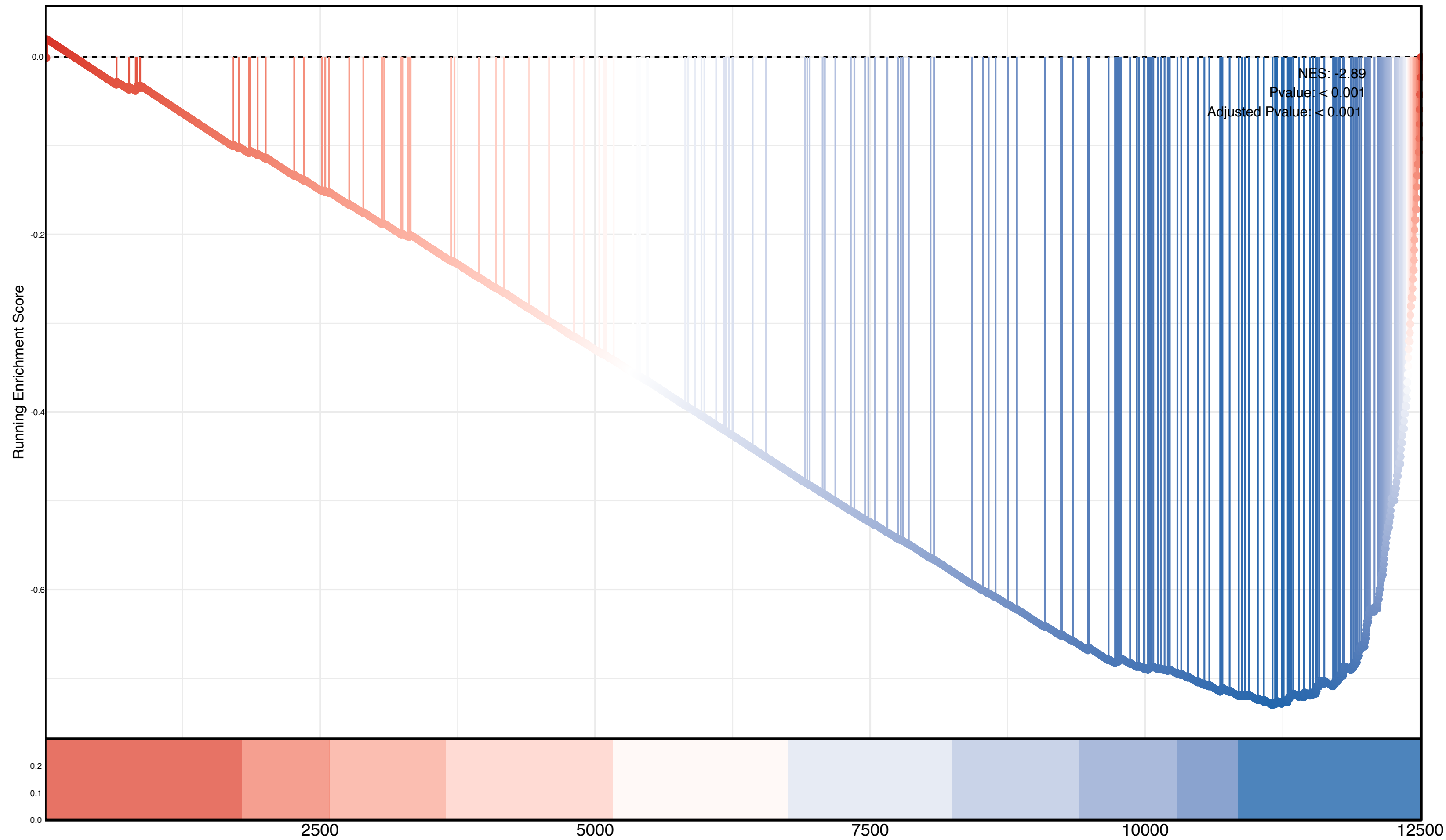
Chromosome Centromeric Region
