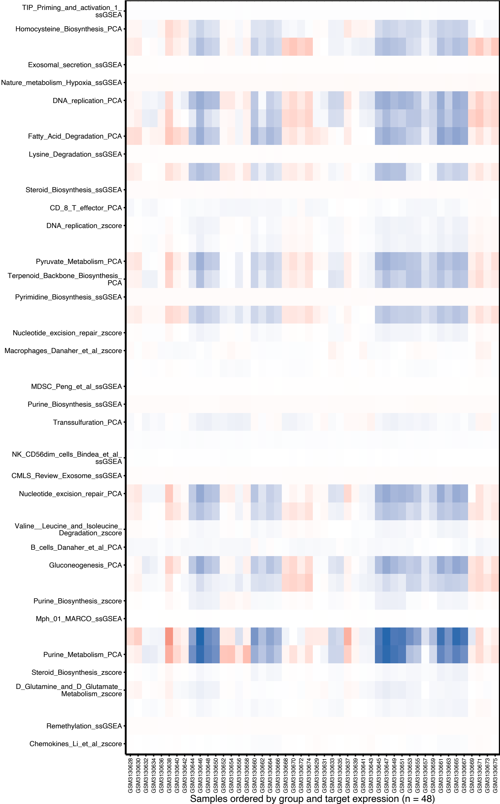
GSE114012_integration all IOBR features heatmap part 003/022
