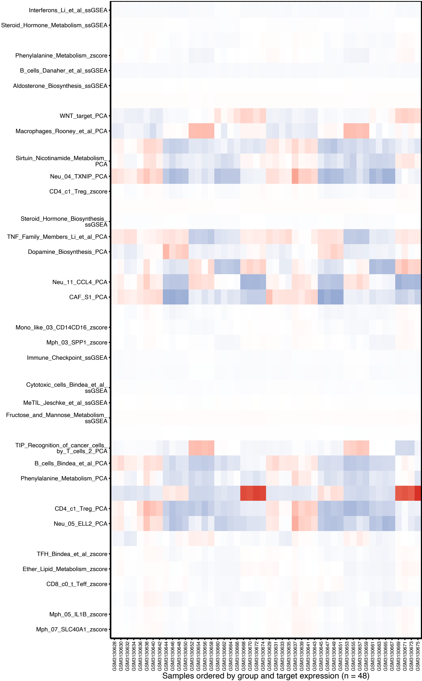
GSE114012_integration all IOBR features heatmap part 015/022
