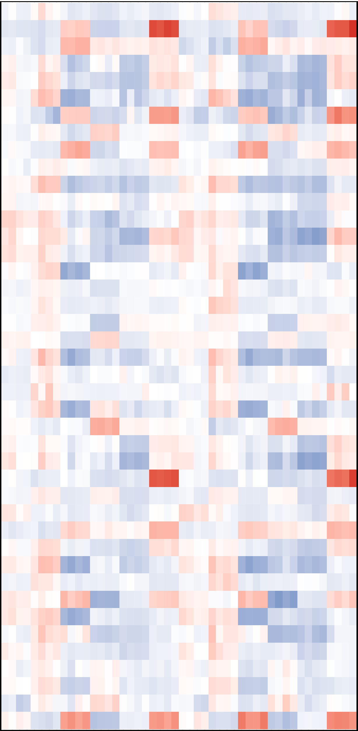
GSE114012_pca all IOBR features heatmap part 004/008
