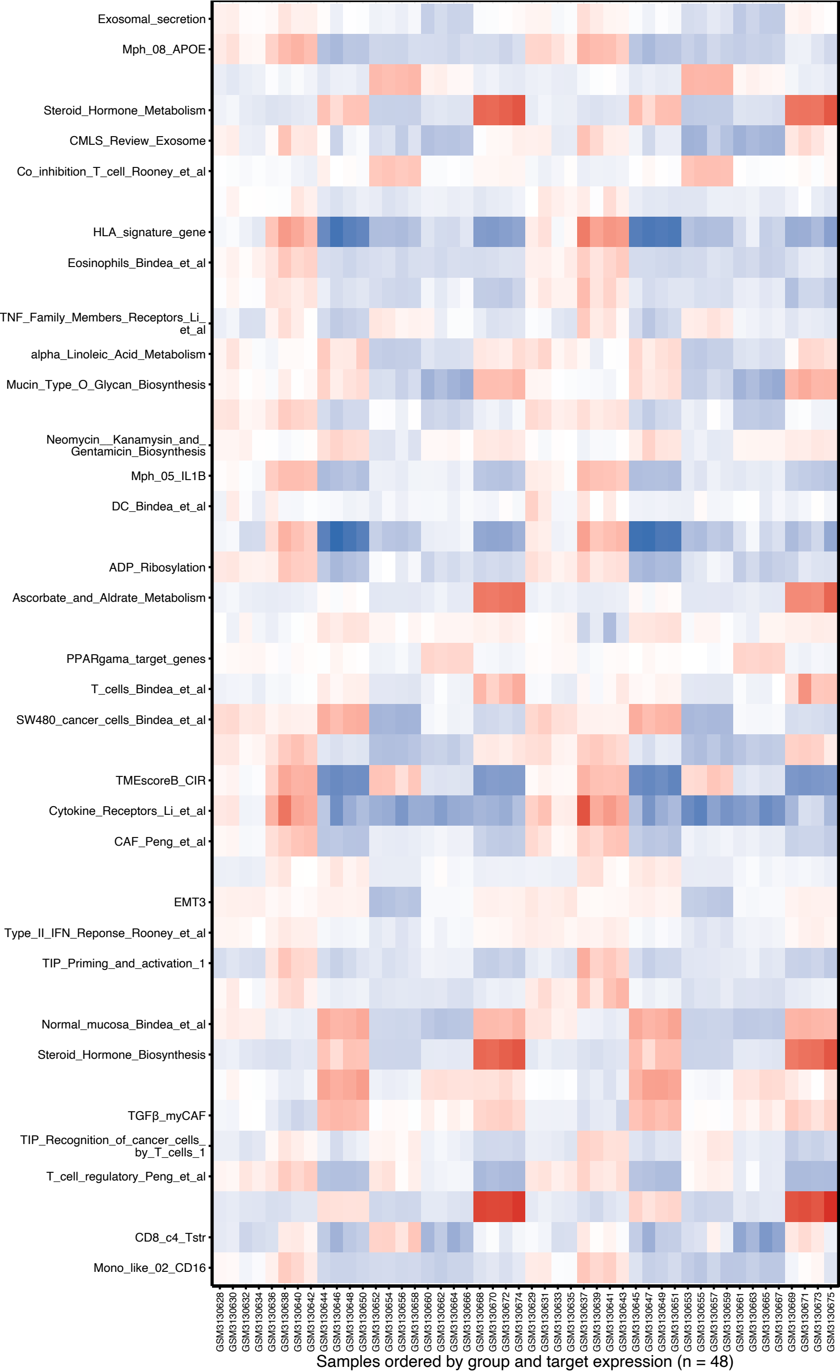
GSE114012_pca all IOBR features heatmap part 006/008
