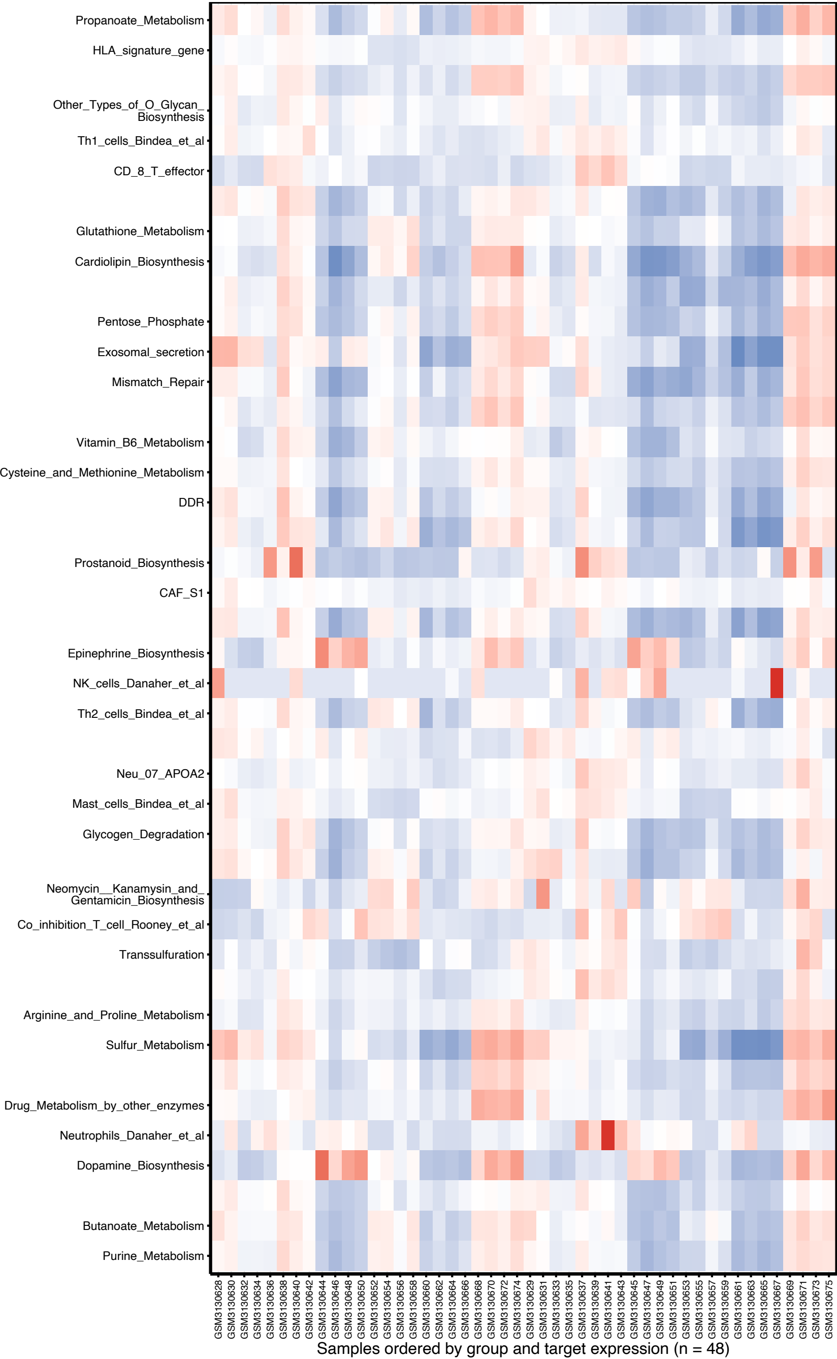
GSE114012_zscore all IOBR features heatmap part 002/008
