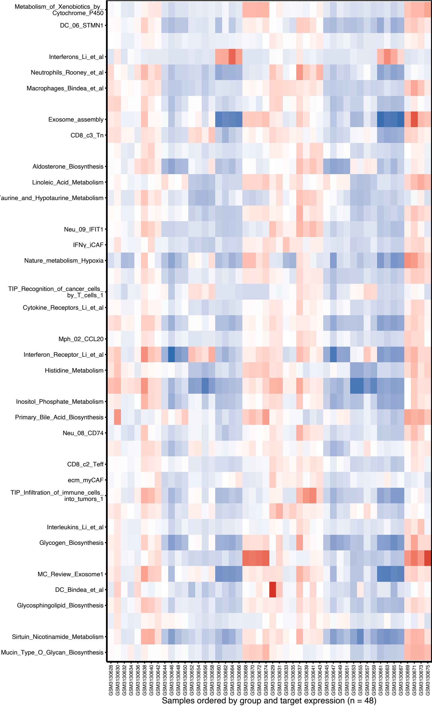
GSE114012_zscore all IOBR features heatmap part 005/008
