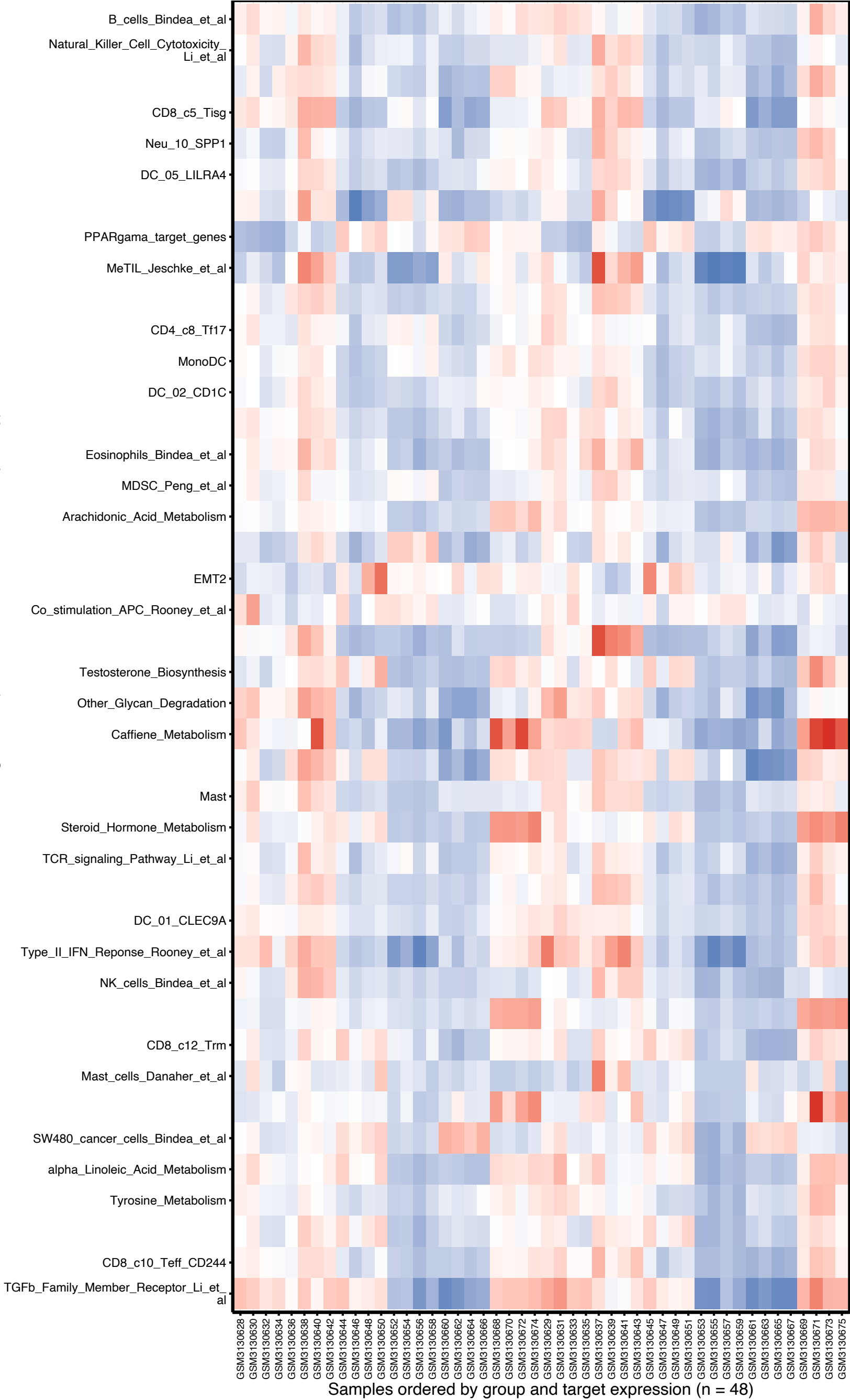
GSE114012_zscore all IOBR features heatmap part 007/008
