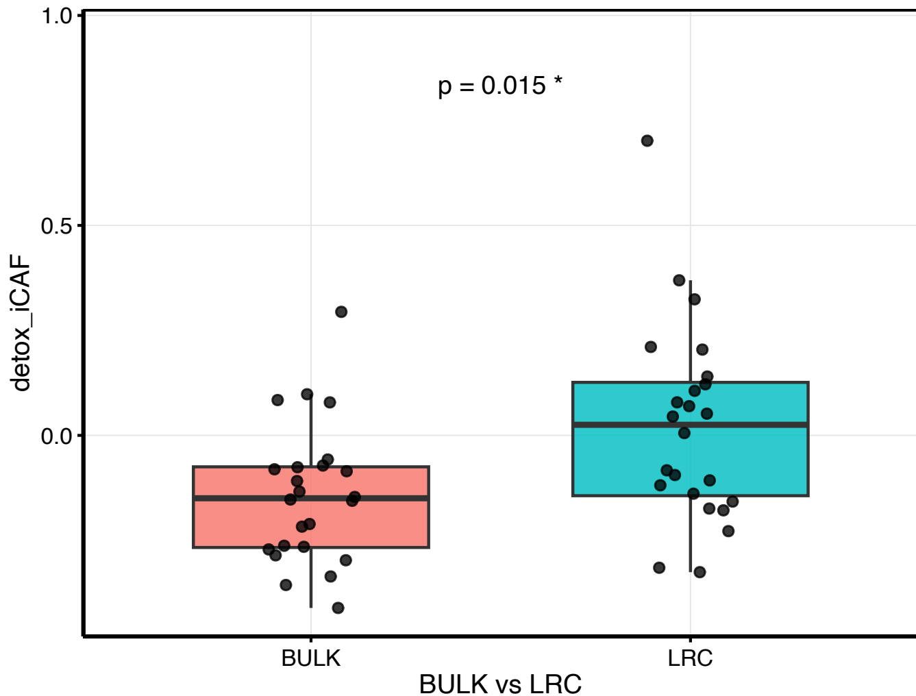
GSE114012_zscore detox_iCAF by BULK vs LRC
