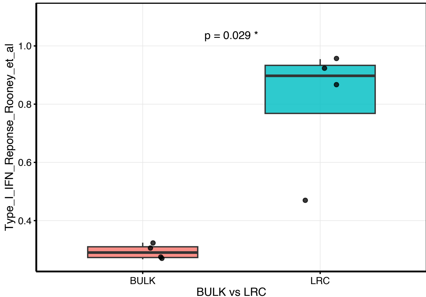
GSE114012_pca Type_I_IFN_Reponse_Rooney_et_al by BULK vs LRC
