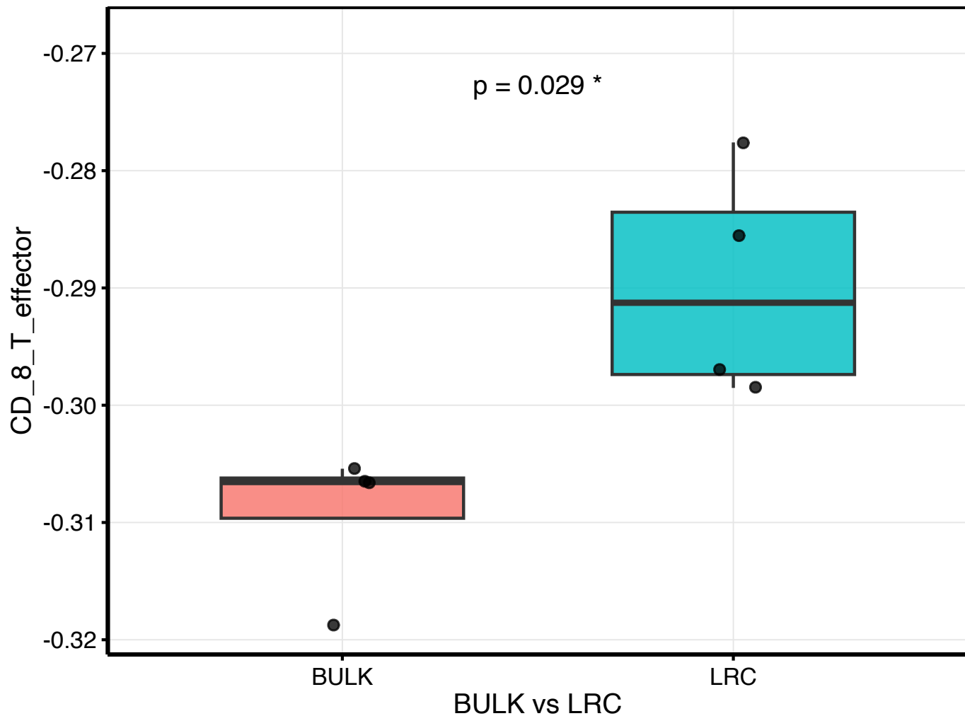
GSE114012_ssgsea CD_8_T_effector by BULK vs LRC
