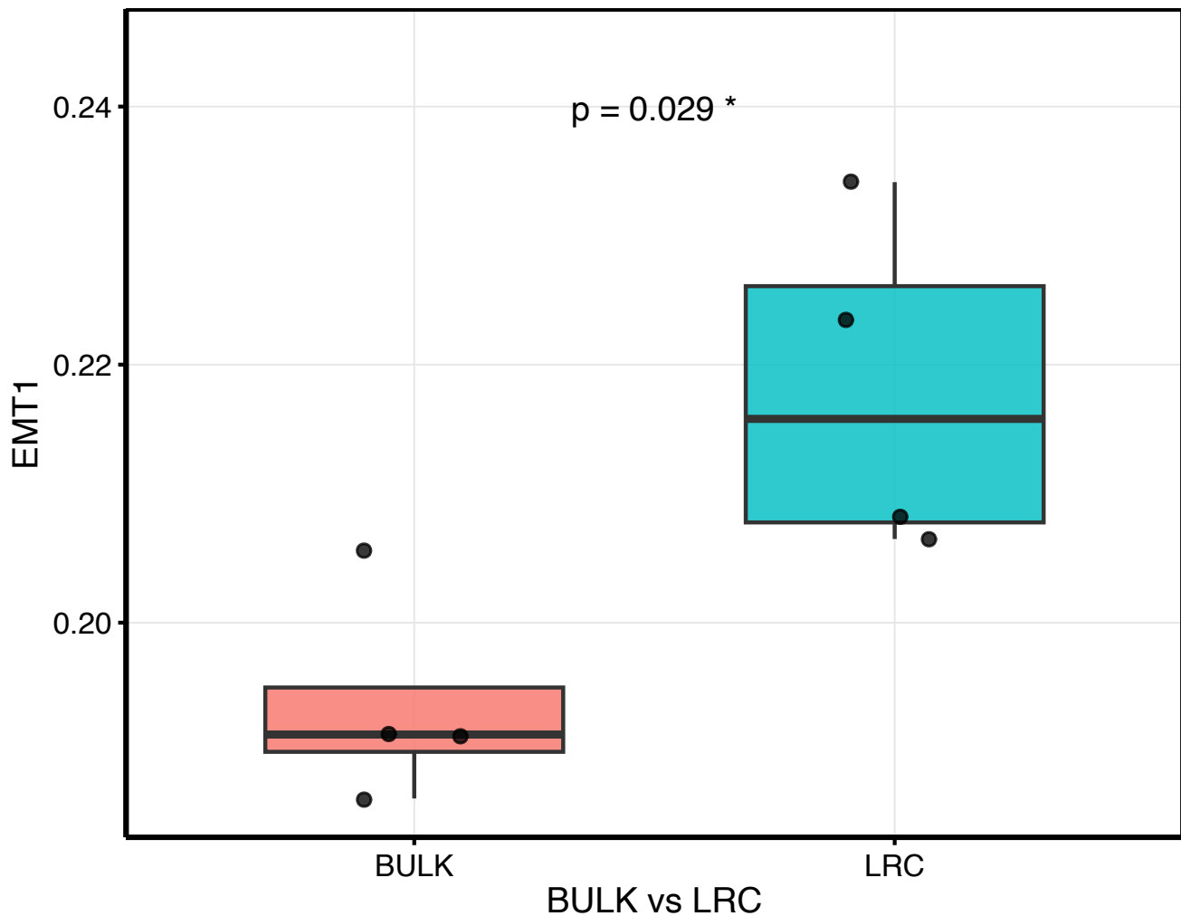
GSE114012_ssgsea EMT1 by BULK vs LRC
