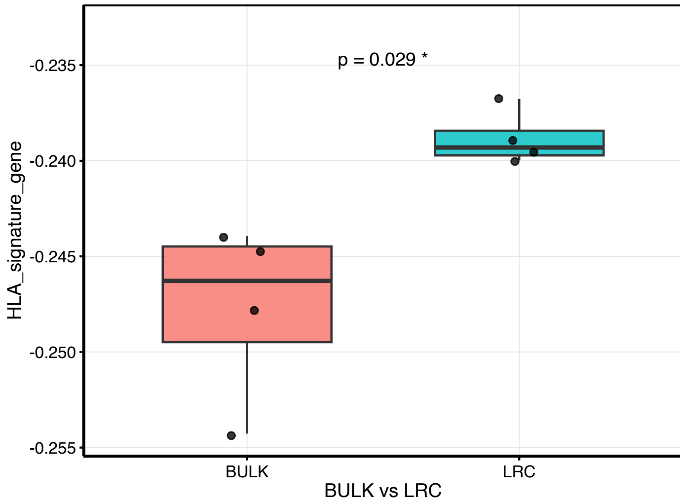
GSE114012_ssgsea HLA_signature_gene by BULK vs LRC
