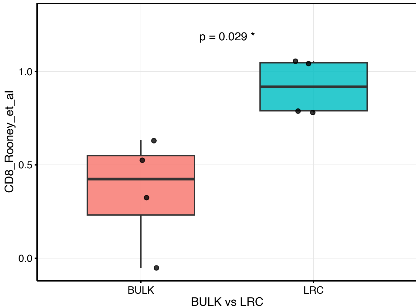
GSE114012_zscore CD8_Rooney_et_al by BULK vs LRC
