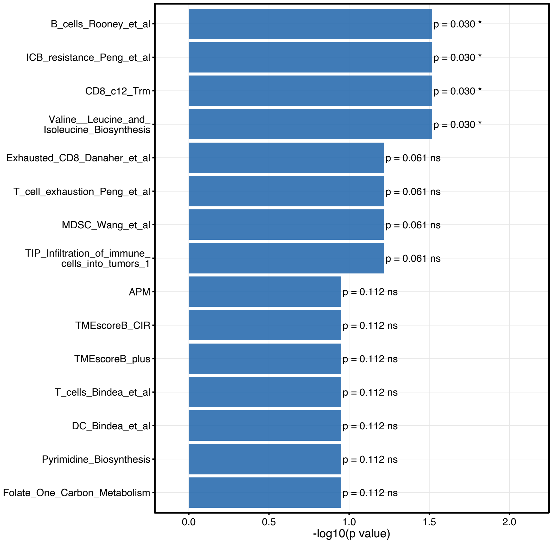
GSE114012_pca group differences: BULK vs LRC
