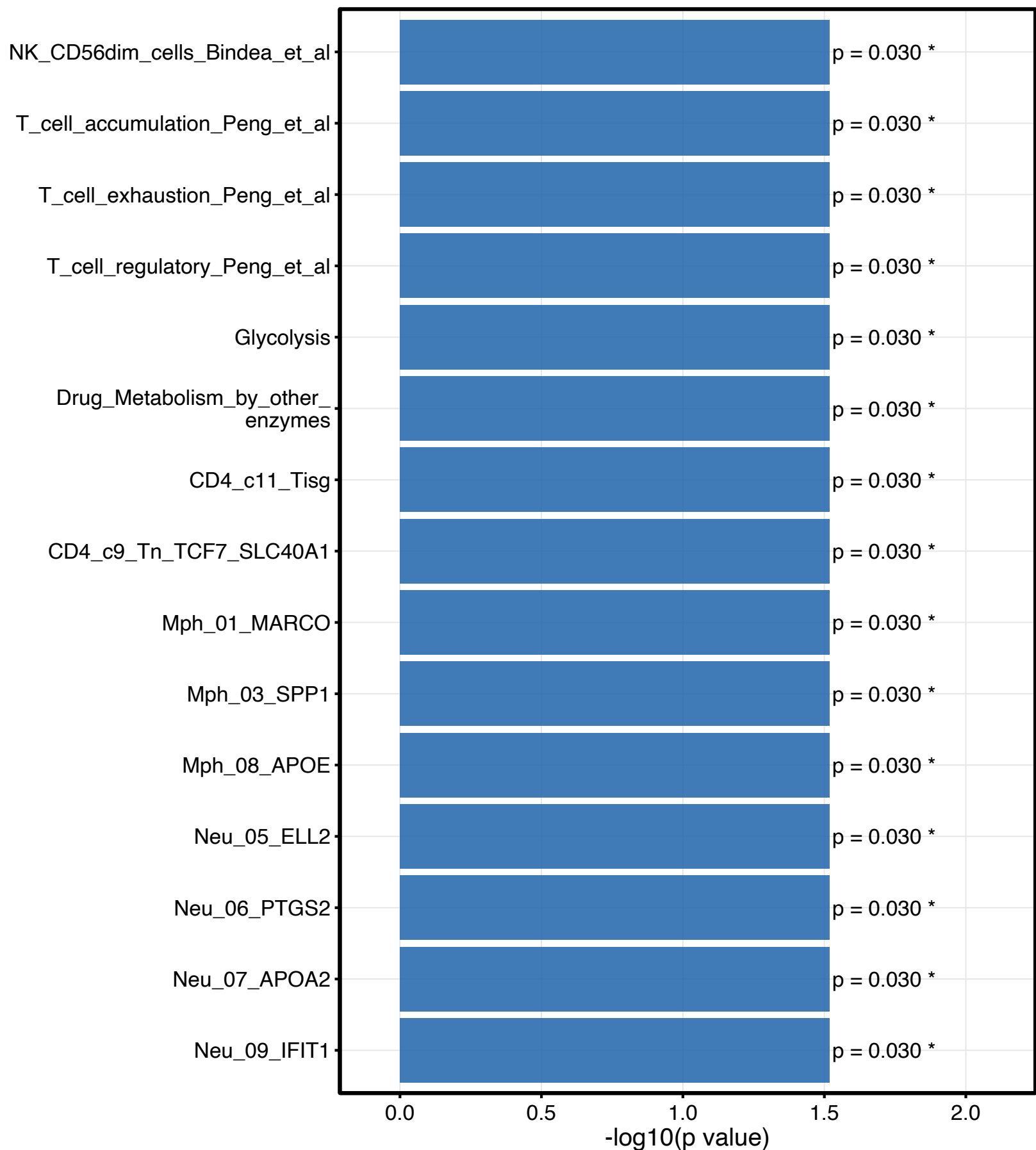
GSE114012_ssgsea group differences: BULK vs LRC
