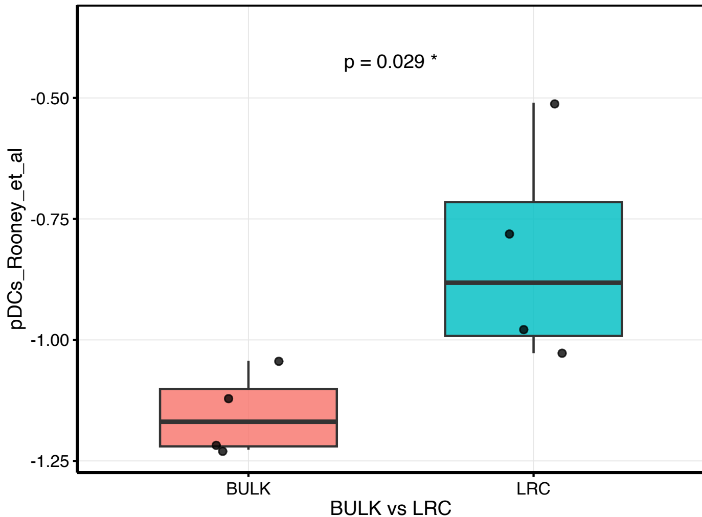
GSE114012_pca pDCs_Rooney_et_al by BULK vs LRC
