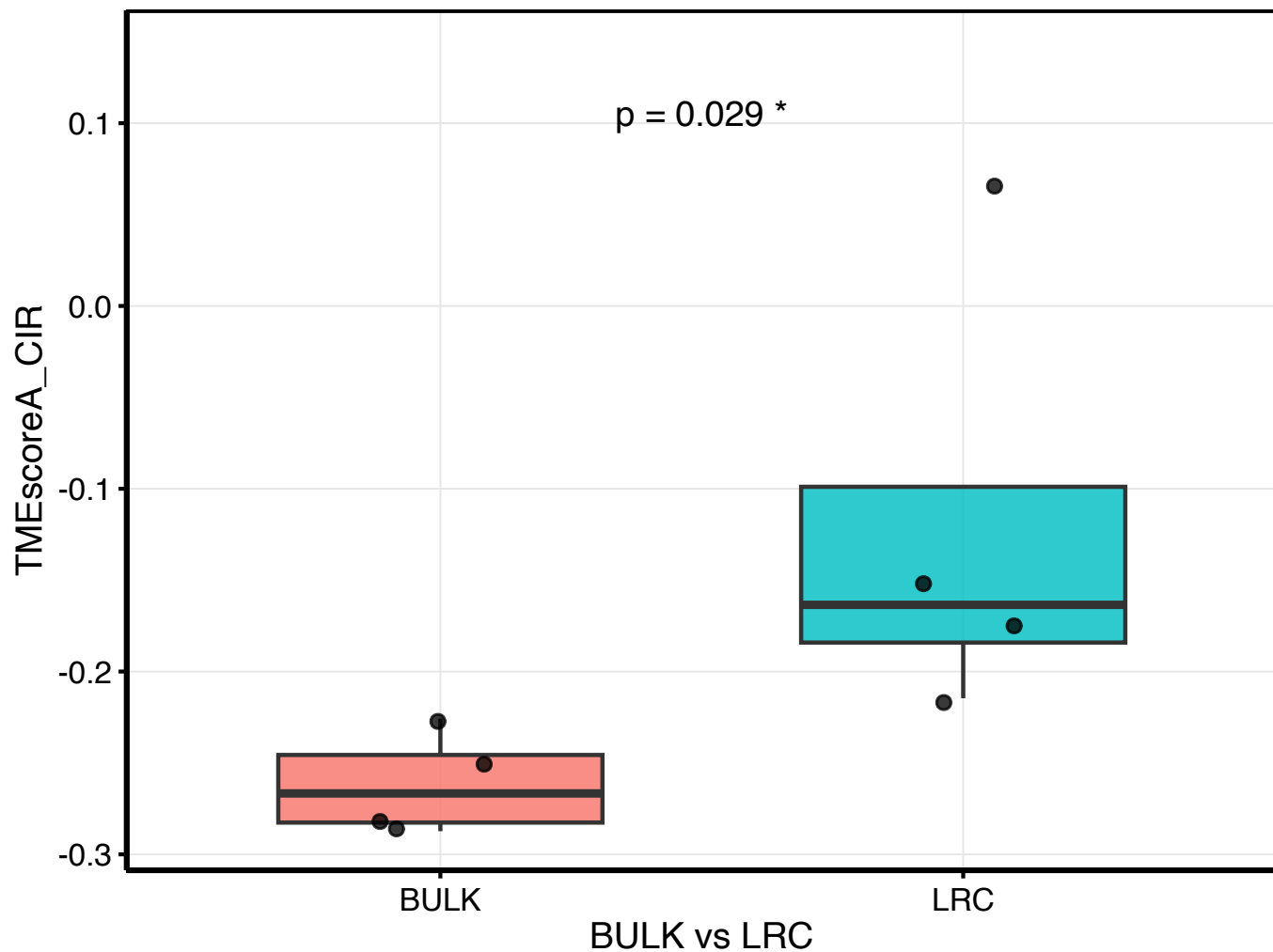
GSE114012_zscore TMEscoreA_CIR by BULK vs LRC
