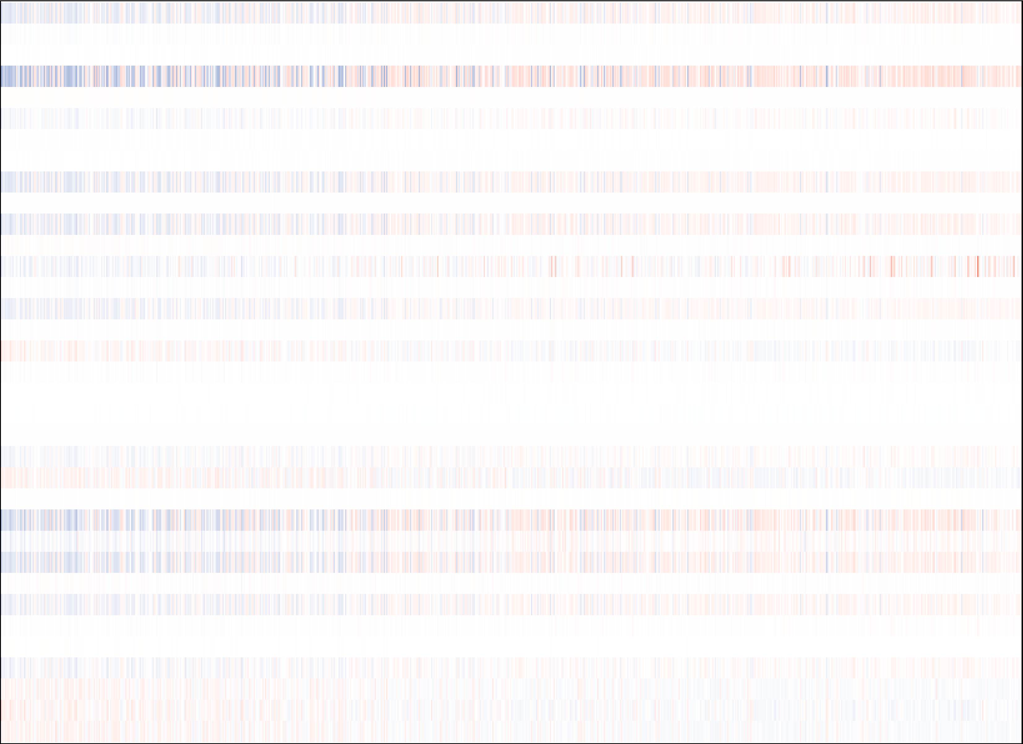
GTEX_COLON_ATF3_integration all IOBR features heatmap part 008/026
