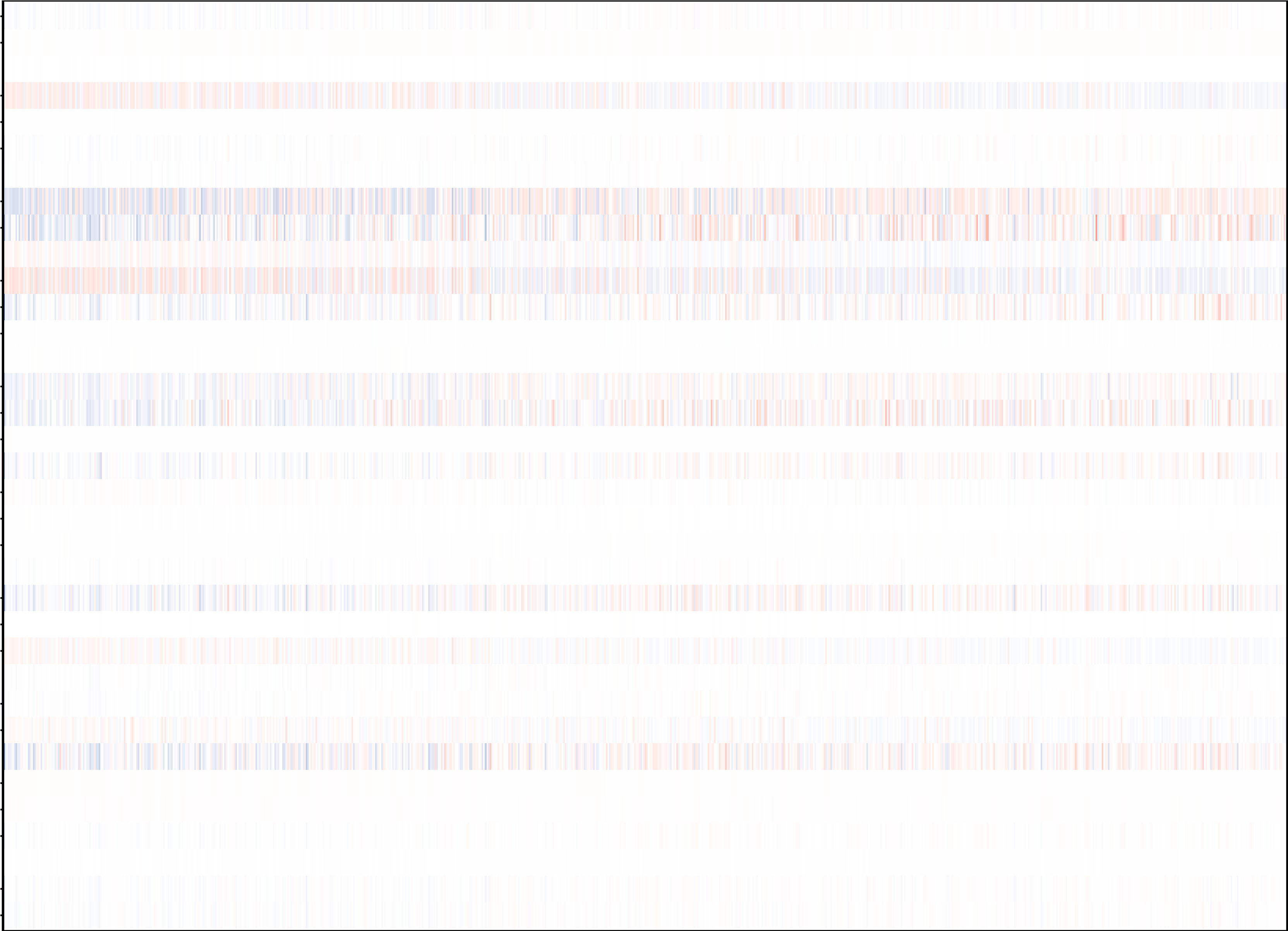
GTEx_COLON_ATF3_integration all IOBR features heatmap part 013/026
