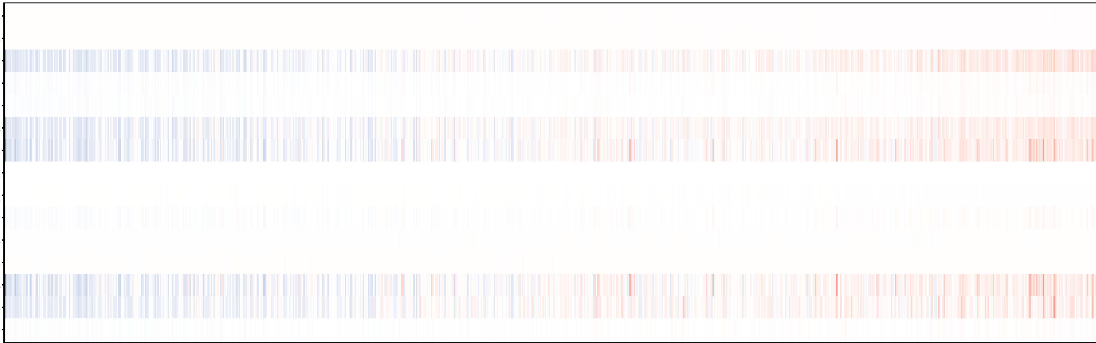
GTEX_COLON_ATF3_integration top feature heatmap
