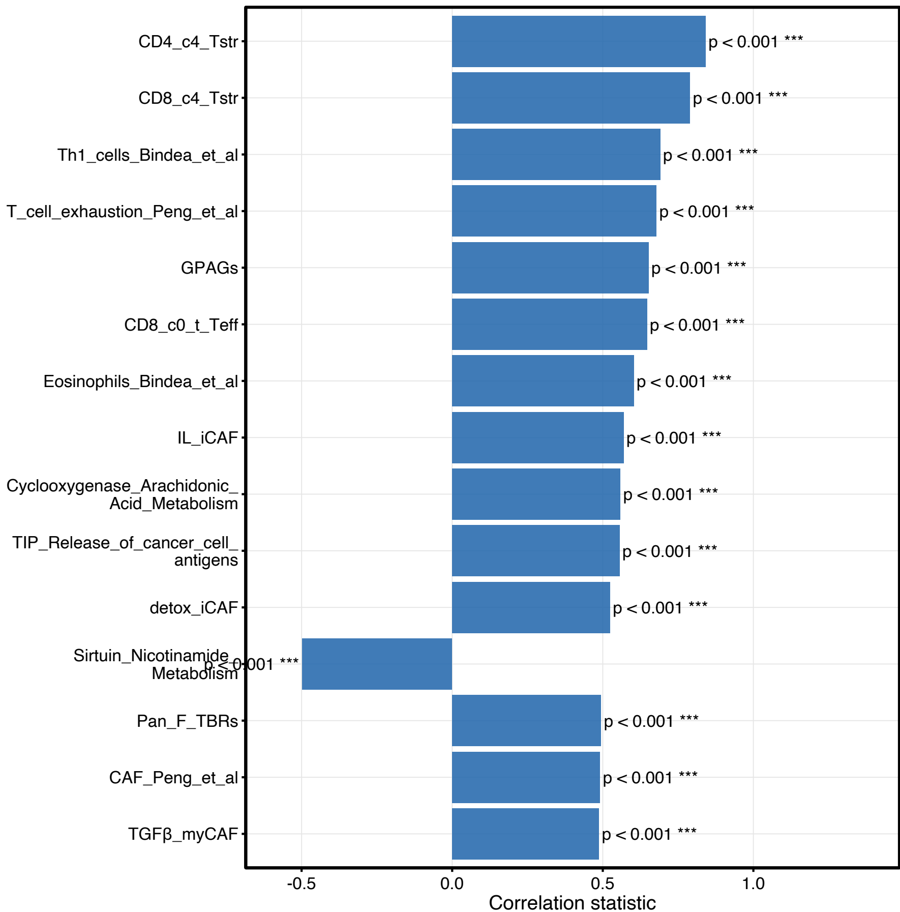
GTEx_COLON_ATF3_ssgsea correlation with target gene
