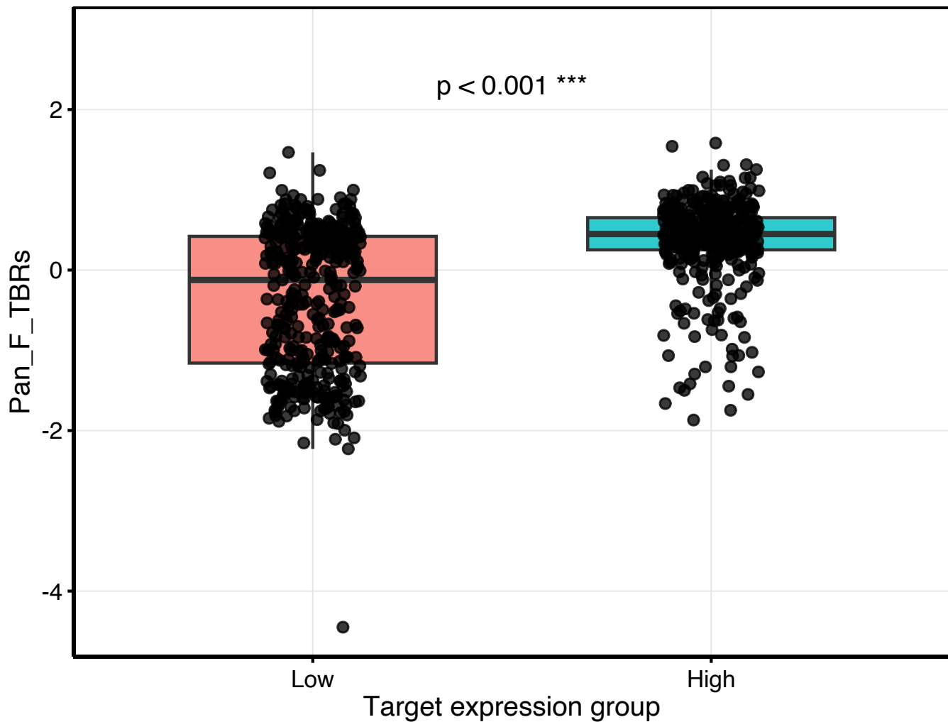
GTEX_COLON_ATF3_zscore Pan_F_TBRs by Target expression group
