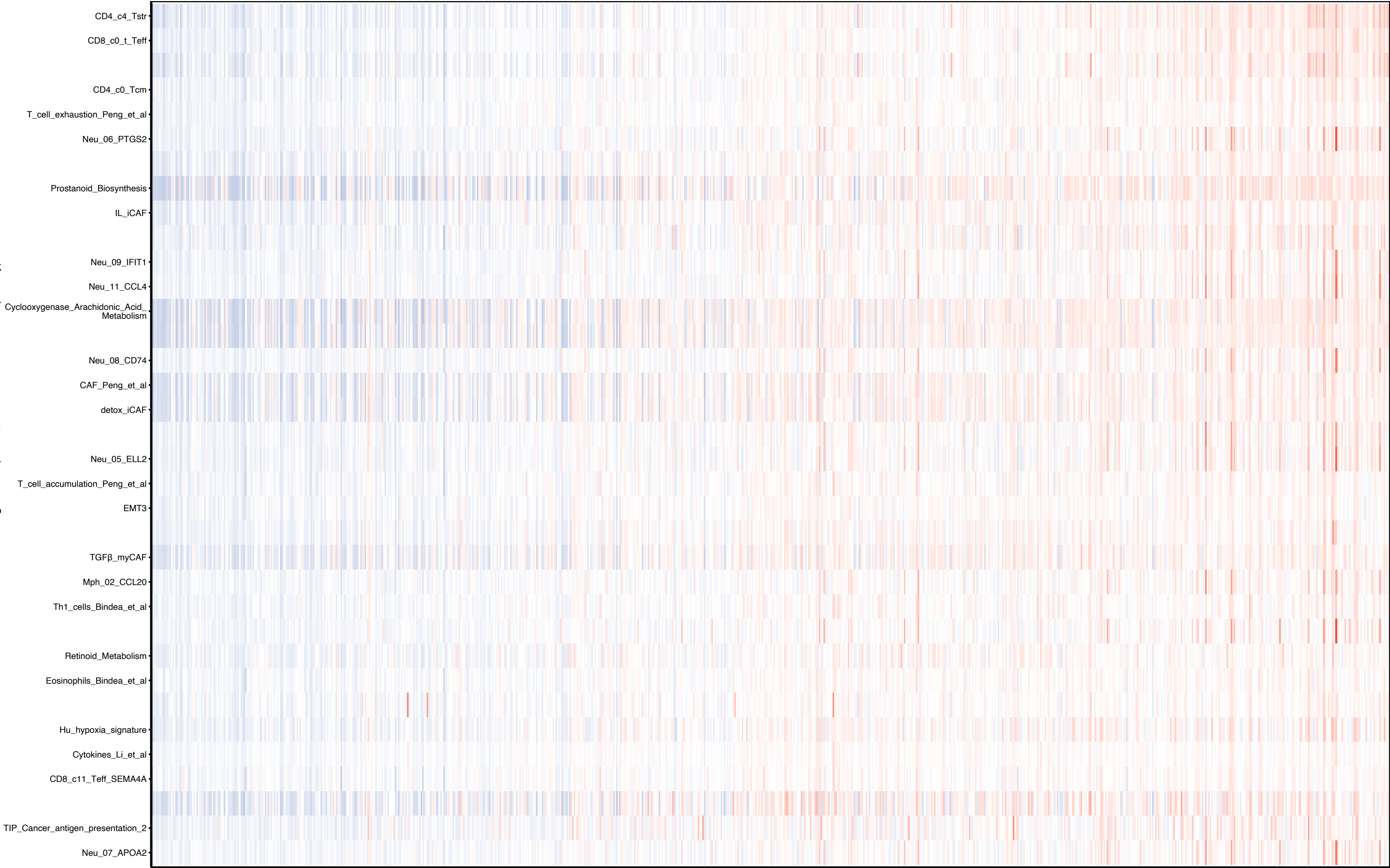
GTEX_COLON_ATF3_zscore all IOBR features heatmap part 001/009
