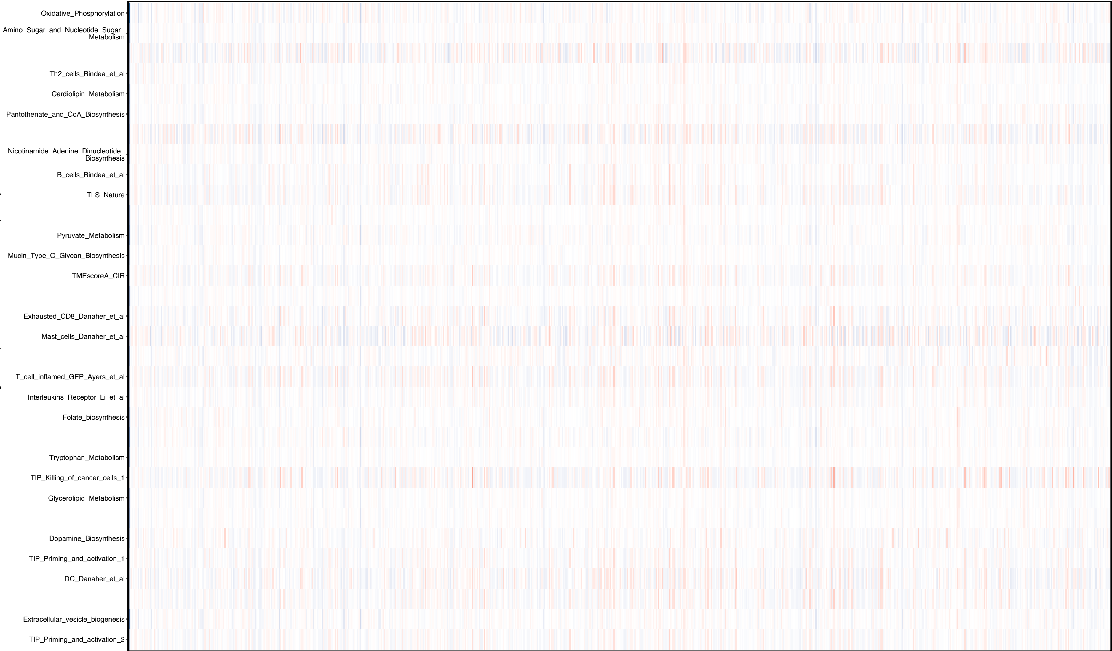
GTEx_COLON_ATF3_zscore all IOBR features heatmap part 009/009
