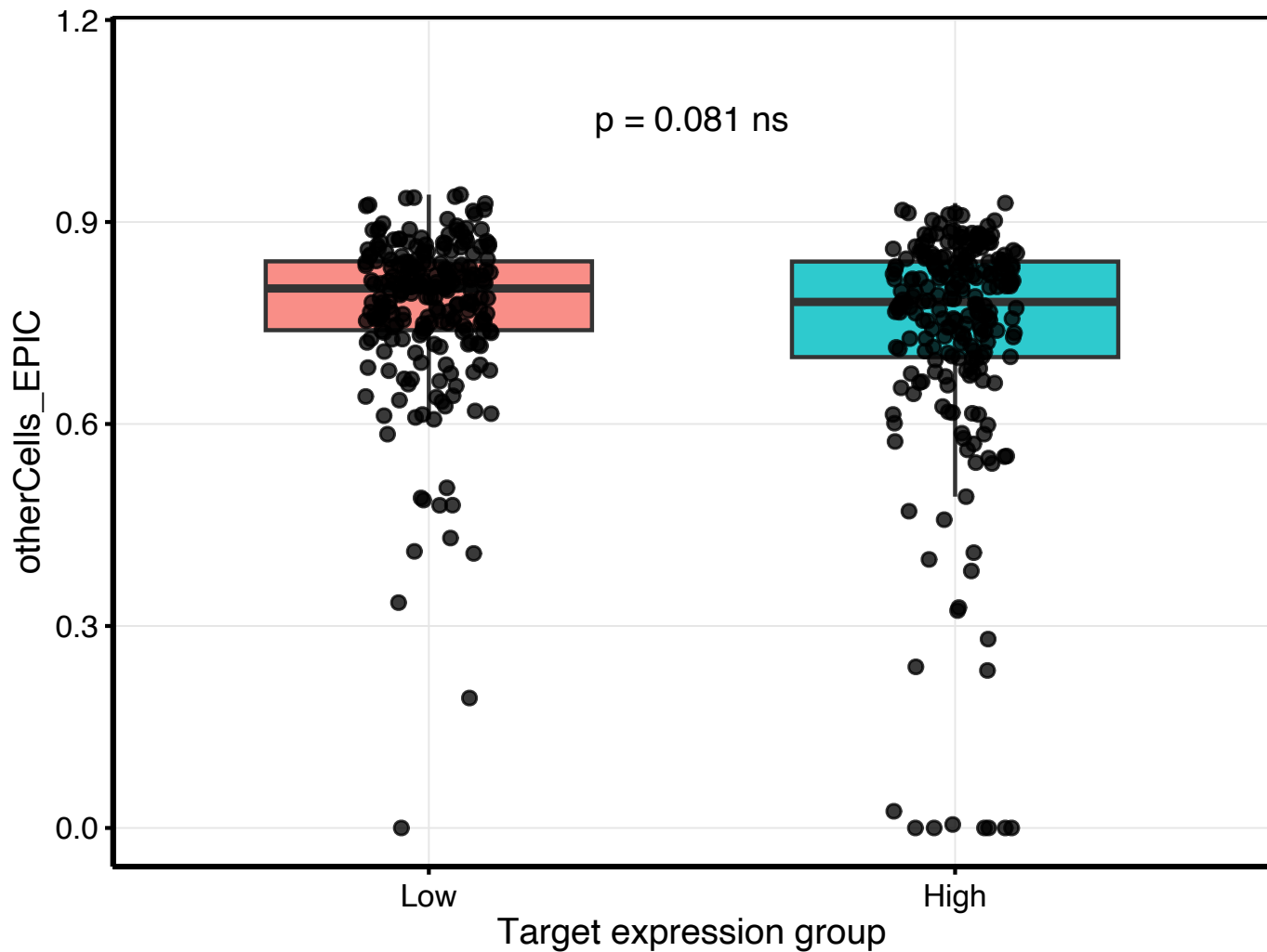
TCGA_COAD_01A_ATF3_epic otherCells_EPIC by Target expression group
